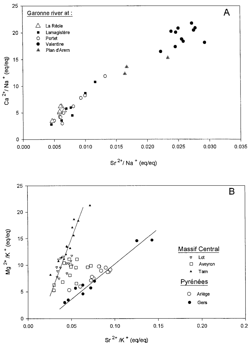
Fig. 4. Variations of ionic \text{Ca}^{2+}/\text{Na}^+ ratios versus ionic \text{Sr}^{2+}/\text{Na}^+ ratios observed in the Garonne waters (A) and ionic \text{Mg}^{2+}/\text{K}^+ ratios versus ionic \text{Sr}^{2+}/\text{K}^+ ratios observed in the main tributary waters (B) during the 1990–1992 period. The ionic \text{Ca}^{2+}/\text{Na}^+ , \text{Sr}^{2+}/\text{Na}^+ , \text{Mg}^{2+}/\text{K}^+ and \text{Sr}^{2+}/\text{K}^+ ratios are in eq/eq.
