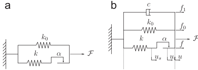
Fig. 3. The Masing model (a) with viscous damping (b).
