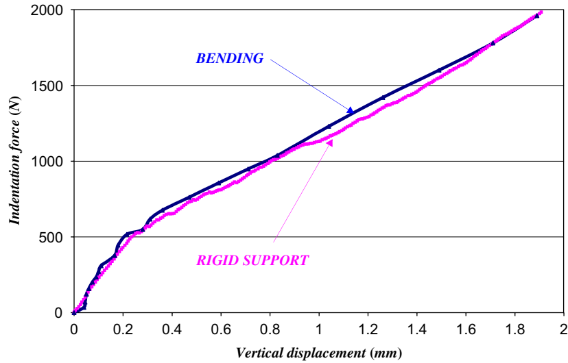
Fig. 17. Comparison of the force/crush experimental curves in the case of rigid support and three-point bending, indenter R = 57.25 mm.
