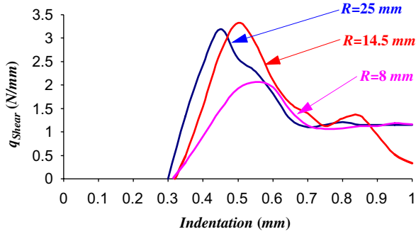
Fig. 8. Peripheral shear force per unit length.
