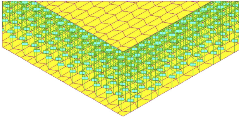
Fig. 4. Sample of discrete modelling of honeycomb core.
