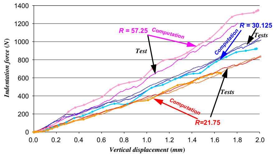
Fig. 12. Test/numerical model correlation in the case of sandwich with thin metal skins.
