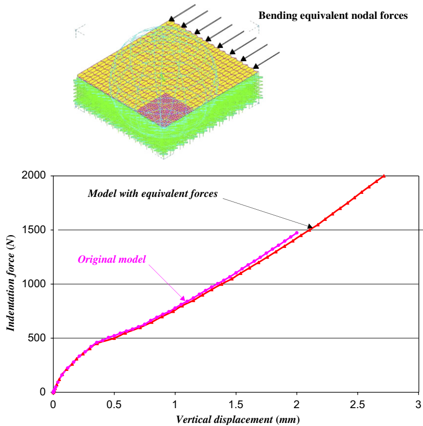
Fig. 18. Adapted model in indentation for bending loads and comparisons between previous modelling and the model with nodal forces, for indenter 21.75 mm.
