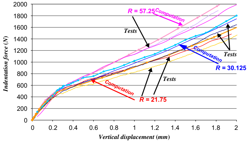
Fig. 13. Test/numerical model correlation in the case of sandwich with thick metal skins.
