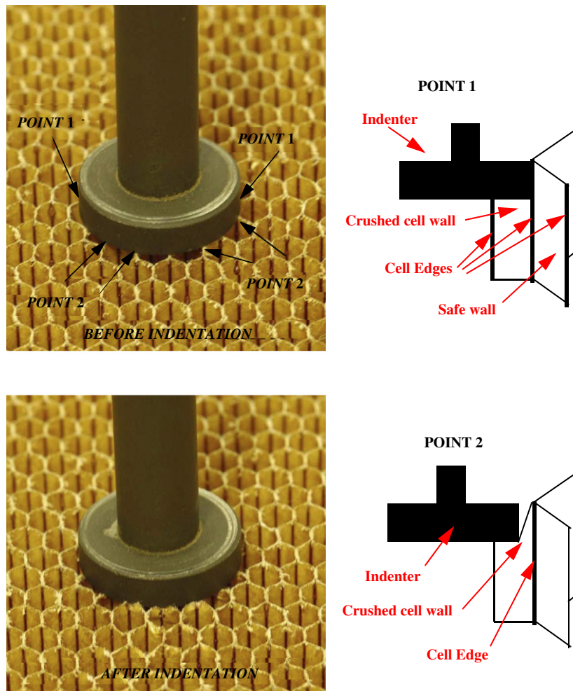
Fig. 6. Description of the indentation test with a cylindrical indenter.
