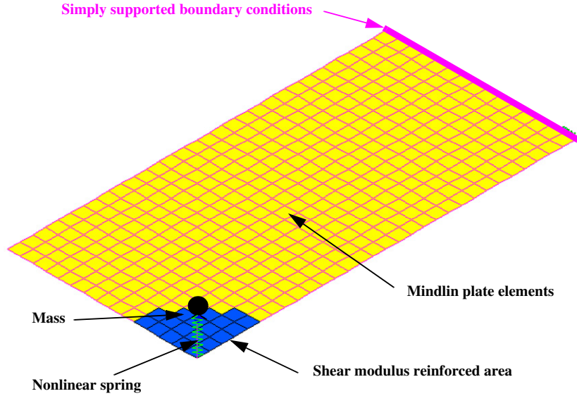
Fig. 20. Spring-mass finite element model.
