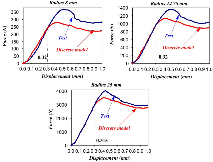
Fig. 7. Experimental contact law with cylindrical indenter and discrete model comparison.
