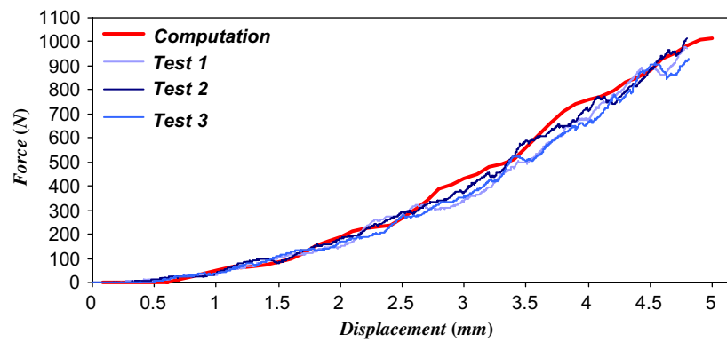
Fig. 10. Comparison between calculation and indentation tests with conical indenter (angle: 18^\circ ).
