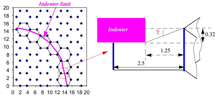
Fig. 9. Geometry for the computation of the limit \gamma .
