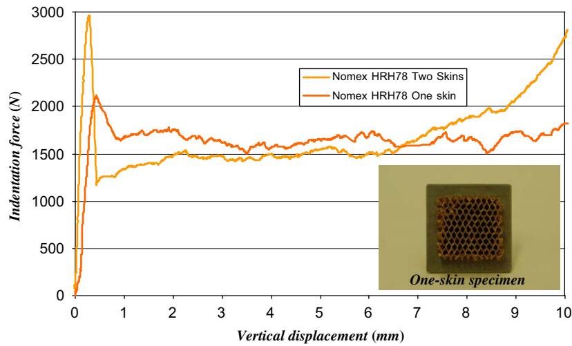
Fig. 2. Compression test curve of the block.
