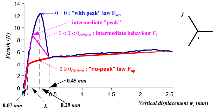
Fig. 5. Generalized crushing law F_{\text{crush}}(w_i, \theta_i) of cell edge i .
