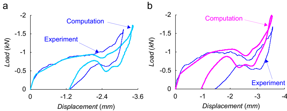
Fig. 21. Dynamic load–displacement law: (a) impactor 30.125 mm and (b) impactor 57.25 mm.
