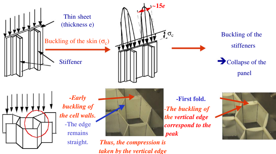
Fig. 3. Analogy with the buckling of stiffened panels.
