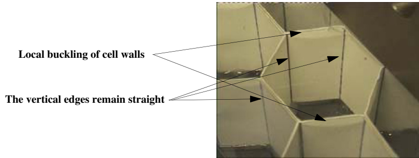
Fig. 1. Mechanism of crushing for a one-skin paper specimen.
