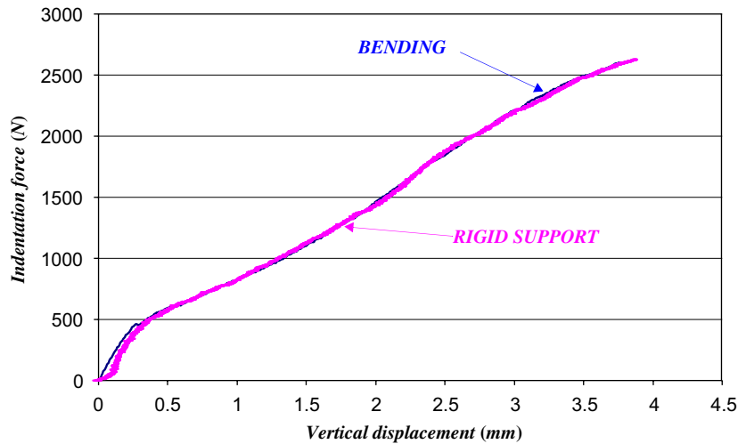
Fig. 16. Comparison of the force/crush experimental curves in the case of rigid support and three-point bending, indenter R = 21.75 mm.
