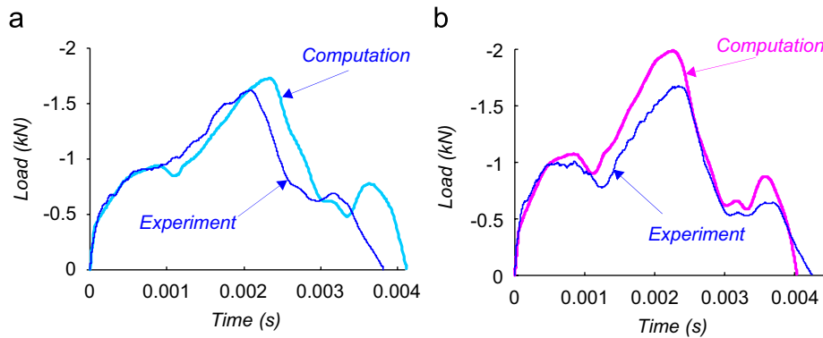
Fig. 22. Dynamic load–time law: (a) impactor 30.125 mm and (b) impactor 57.25 mm.
