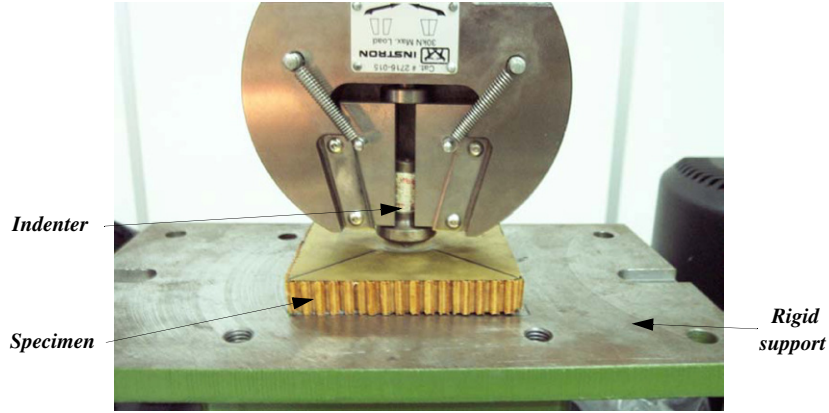
Fig. 11. Description of the indentation tests on sandwich specimens.
