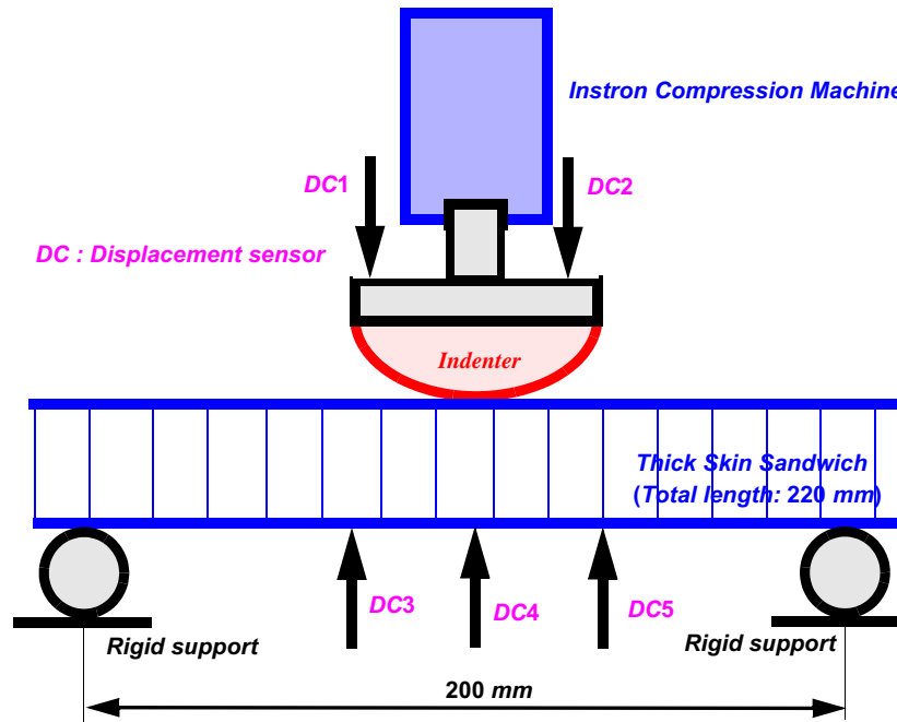
Fig. 15. Three-point bending test principle.
