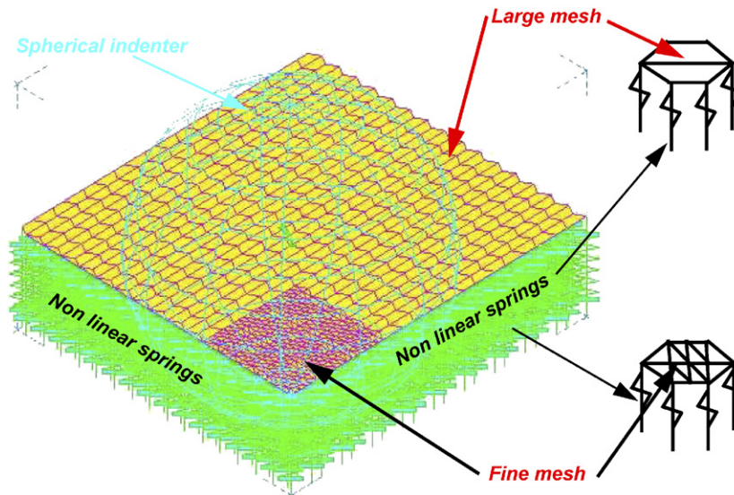
Fig. 14. Finite element modelling of the indentation problem on sandwich with thin metal skins.
