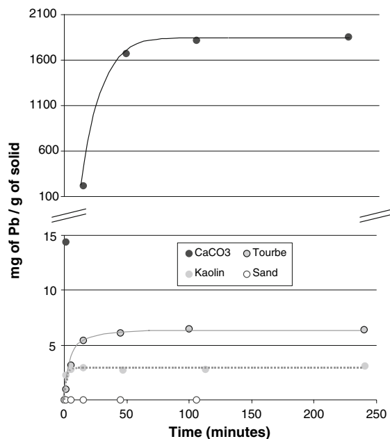
Fig. 4 Pb extraction quantity ( \text{mg Pb g}^{-1} \text{solid} ), by the different constituents of the artificial soil versus time
