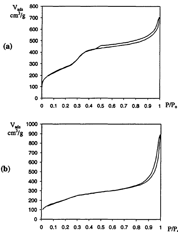
Fig. 4 Isotherms of adsorption and desorption of N 2 (gas) after calcination of the samples A (a) and C (b). Correspondence to liquid adsorbed volume usually used, V_{ads} in \text{cm}^3 \text{g}^{-1} will be obtained by multiplying the Y axis values by the factor 0.001547.
