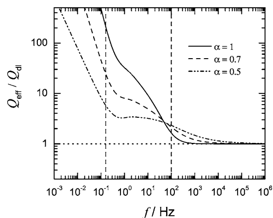
Figure 6. Effective CPE coefficient defined by Eq. 7, scaled by the input value of the double-layer CPE coefficient, as a function of frequency with \alpha as a parameter for the Randles circuit presented as Fig. 1a.
