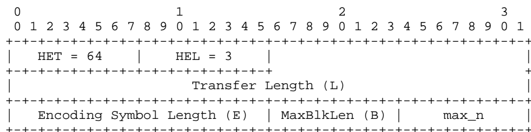
Figure 6: EXT FTI Header Format with FEC Encoding ID 5
