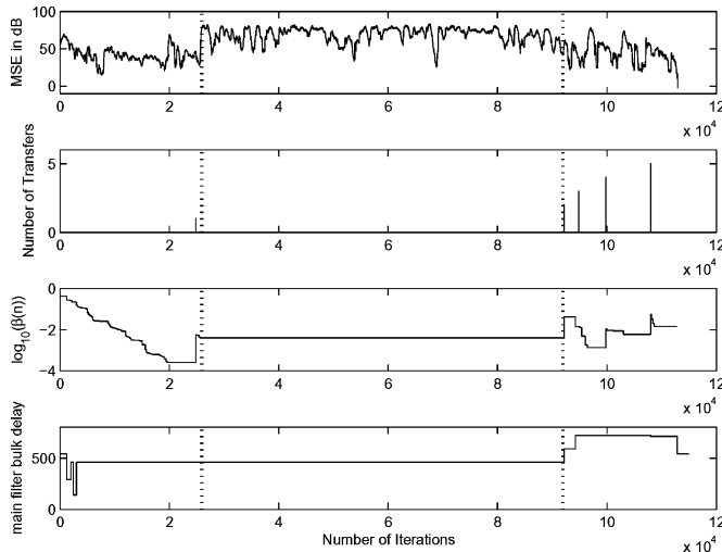
Fig. 10. Performance of conventional EC. (Top) MSE. (Second) Number of transfers from the shadow filter to the main filter. (Third) 10 \ln_{10}(\beta) . (Bottom) Main filter bulk delay.
