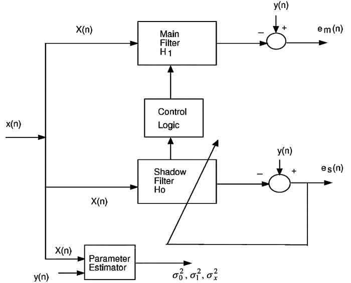
Fig. 1. Basic EC structure.
