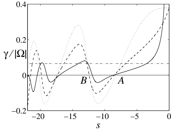
FIGURE 7. Ratio of the strain rate \gamma to the vorticity \Omega along the central isopycnic line. s is the curvilinear coordinate originated at the saddle-point, approximated here as the point of maximum \gamma . The dotted, dashed and solid lines correspond respectively to C_\rho = 0 , C_\rho = 0.1 and C_\rho = 0.5 . The dashed-dotted line denotes a threshold value of 0.065 and A , B represent the first positions with zero strain rate starting from the saddle point.
