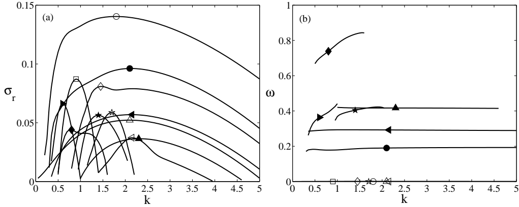
FIGURE 3. (a) Growth rate and (b) temporal frequency vs. spanwise wavenumber k for the maximum-amplitude state ( t = 24 ) of the nonlinear KH wave with C_\rho = 0 and Re = 300 . The symbols on each branch denote the fastest growing mode.
