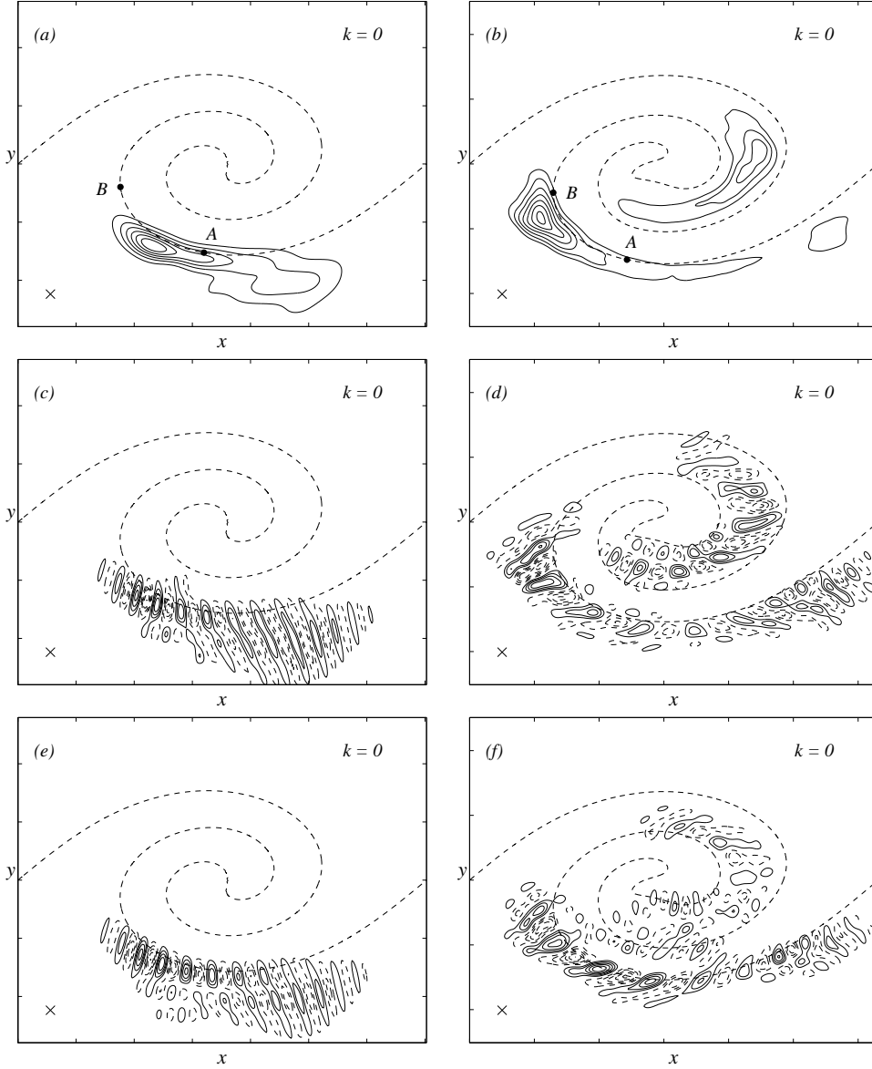
FIGURE 6. Structure of the most amplified two-dimensional baroclinic Kelvin-Helmholtz mode ( \times ) at C_\rho = 0.1 (first column) and C_\rho = 0.5 (second column). The contours represent iso-levels of energy in (a) and (b), iso-levels of spanwise vorticity in (c) and (d), iso-levels of density in (e) and (f). The mode characteristics are \sigma_r = 0.0799 , \omega = 9.45 for C_\rho = 0.1 and \sigma_r = 0.237 , \omega = 4.6 for C_\rho = 0.5 . Perturbations are normalised to have a unitary energy. The contour increments are respectively u_0^2/4 , 1/2t_0 and \Delta\rho/2 for the energy, vorticity and density fields. The dashed levels correspond to negative values and the dashed line denotes the central isopycnic line of the base flow. Points A and B are defined in figure 7.
