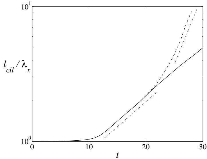
FIGURE 11. Temporal evolution of the length \ell_{cil} of the central isopycnic line normalised by \lambda_x . The dashed and solid lines correspond respectively to the case with and without the baroclinic secondary instability. The dashed-dotted lines measure respective exponential growth rates \sigma_\ell = 0.24 and \sigma_\ell = 0.085 .
