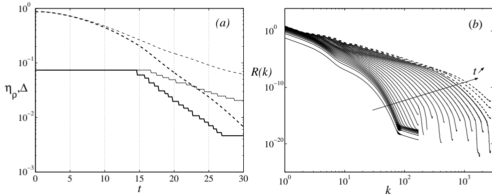
FIGURE 1. (a) Characteristic length scale of the density gradient \eta_\rho (dashed lines) and the smallest length scale properly resolved by the dealiased pseudo-spectral approach \Delta (solid lines) for C_\rho = 0.5 . Thick lines correspond to an infinite Schmidt number, Sc = \infty , and thin lines to Sc = 1 . (b) Time spreading of the density variance spectra for C_\rho = 0.5 and Sc = \infty . Dashed spectra correspond to t = 28, 29 and 30 when the constraint in spatial resolution, \Delta < \min(\eta_\rho)/3 , is released.
