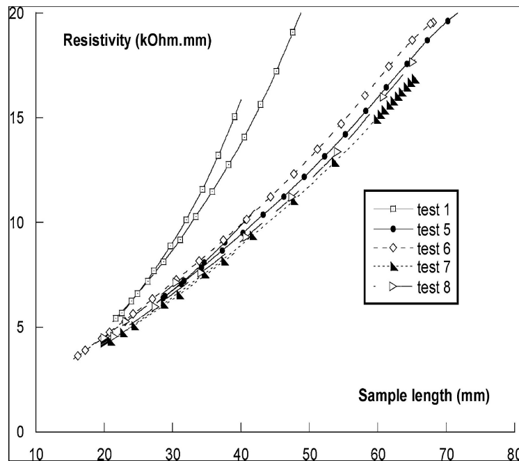
(Fig. 7). It is worth noticing that the sample electrical resistivity is a reversible function of the sample length. The same curves are obtained with humid rawcotton. In the case of steel wool, the shape of the curves obtained is different and some irreversibility appears (Fig. 8). This particular behaviour may be due to the local pliability of these fibres and to the irreversibility of such plastic deformation. However, the results obtained for the carbon nano tubes are similar to those of steel wool and more difficult to explain.
