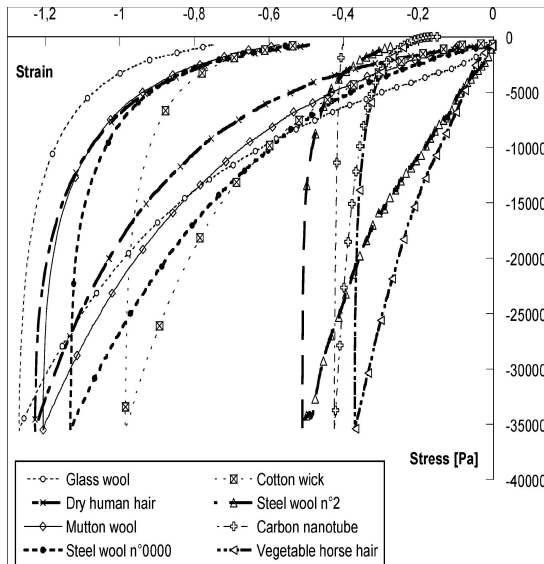
Fig. 5 gathers compression curves obtained on the various materials tested in this study. These data about the mechanical behaviour of various entangled fibres have been obtained during compression tests carried out at a 6 mm/min displacement rate. Unload is performed at the same rate as soon as the maximum load (here 100 N that corresponds to a 35370 Pa stress) is reached. The shape of the curve is comparable for all the materials tested. A remanent strain is noticed for all the materials, due to the rearrangement of the fibres during this first compression cycle. Glass wool has the larger residual strain, which is likely to be due to the regular shape of the fibres and to their smooth surface, which minimize friction stresses. Human hairs are also elastic fibres with both regular shape and surface so that entangled human hair achieved large compression. Curves obtained for raw cotton fibres and sheep wool are similar and we choose to plot only the mutton wool data on Fig. 5. The humid raw cotton achieved slightly higher compression than the dry one (in average 115% instead of 105%). Water content is known to increase elasticity of the cellulose as well as that of the keratin (human hair). Thus a higher humidity rate is supposed to enhance the bending properties of these organic fibres and consequently improving their capacity to be compressed. However, this is a minor effect as compared to the scattering of the results, which is inherent to the initial morphology of the set of entangled fibres (microstructural effect). This humidity of the fibres was needed to achieve electrical measurements as detailed in another paragraph. For the wick of cotton, we investigated the effect of the length of the wick on the mechanical response of the sample in compression. When the wicks length is below the diameter of the cylinder, no size effects can be reported whereas they become noticeable when wicks are long compared to the diameter of the device. Compression rate achieved at the same load are then smaller with longer wicks. This point means that the results we get with steel wool and cotton wick can be dependent on the size of the apparatus contrary to the results obtained for the other fibres tested.
