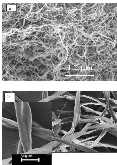
Figure 1 Microstructure of the fibres used in the study, as observed by SEM: (a) carbon nanotubes, (b) raw cotton fibres.
