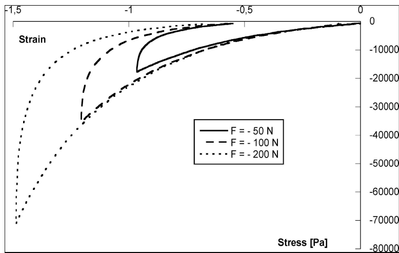
Fig. 6 for mutton wool, increasing the load level gives the same master curves and furthermore the residual strain appears to be quite constant for the elastic fibres tested in that conditions (muttonwool, rowcotton, wick of cotton, vegetable horsehair) whereas it is clearly dependent on the load level reached for the two steel wools tested. This point clearly indicates that the macroscopic compression curves obtained is due to the morphology of the assembly and to the relative motion and friction of the fibres. The non-linearity of the curve cannot be explained solely by the individual behaviour of the fibre. Since the data available (glass wool, carbon nano tube) and the traction tests performed in our laboratory on isolated fibres (human hair, mutton wool, raw cotton) confirm that these fibres follow a linear elastic behaviour in the beginning of the traction tests. On the other hand, steel wool fibres have plastic zones with permanent strain before any test (Fig. 2b). These knees can promote strain localisation provided that the strain hardening of the corresponding steel is weak. 3.2. Electrical resistance Compression tests have been carried out several time on the same sample (carded between each test) on mutton
