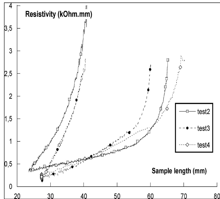
Figure 9 Humid raw cotton fibres of 3 cm. Cyclic compression tests until 100 N at 6 mm/min. occur and the assembly would keep its microstructure. As the matted fibres have taken a certain shape after the first compression their ability to be compressed is largely reduced for the next cycle. This stabilisation of contact between fibres is confirmed by the electric measurement.
