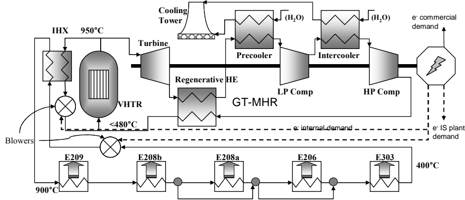
Fig. 1. Cogeneration of Heat and Electricity with a VHTR nuclear reactor (600 MW)
