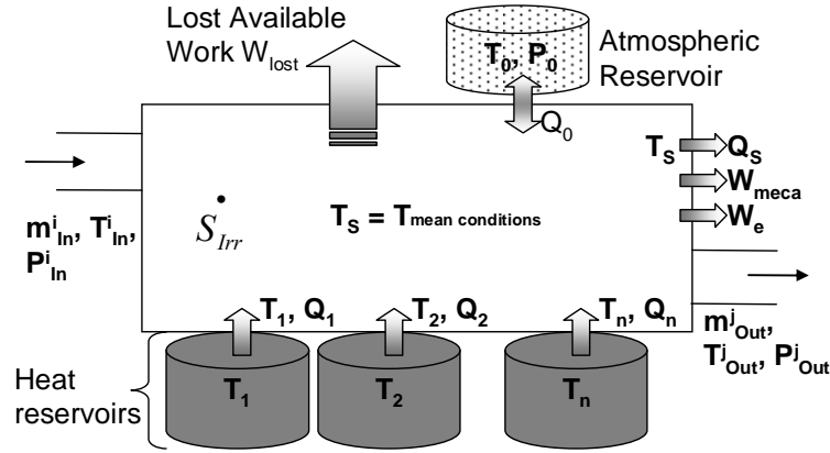
Fig. 2. Open thermodynamical machine producing various type of useful energy
