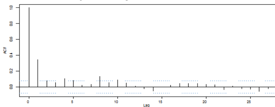
Fig. 1. ACF Graph for Stock Return Series
