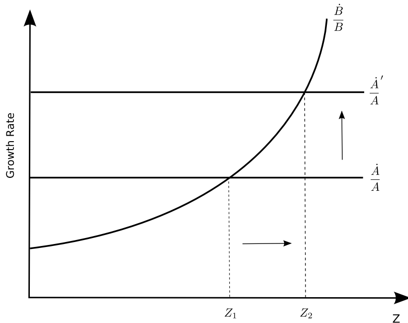
Figure 4: Financial development and changes in the steady state ratio Z = \frac{\dot{A}_t}{\dot{B}_t} .
