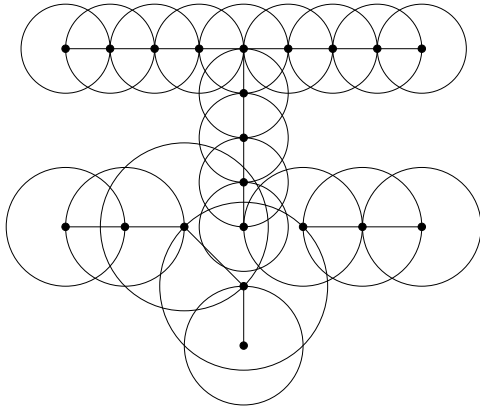
Figure 3.7: An unwanted connection scenario.
