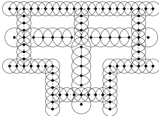
Figure 3.6: The resulting set of stations, with a minimal configuration and the induced communication graph.
