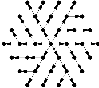
Figure 4.11: The 3-comb, with an MST range assignment.
