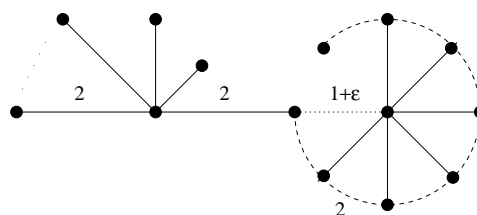
Figure 4.10: ... and an adaption for KRUSKAL.
