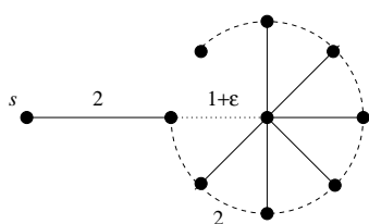
Figure 4.9: A tight instance for PRIM...
