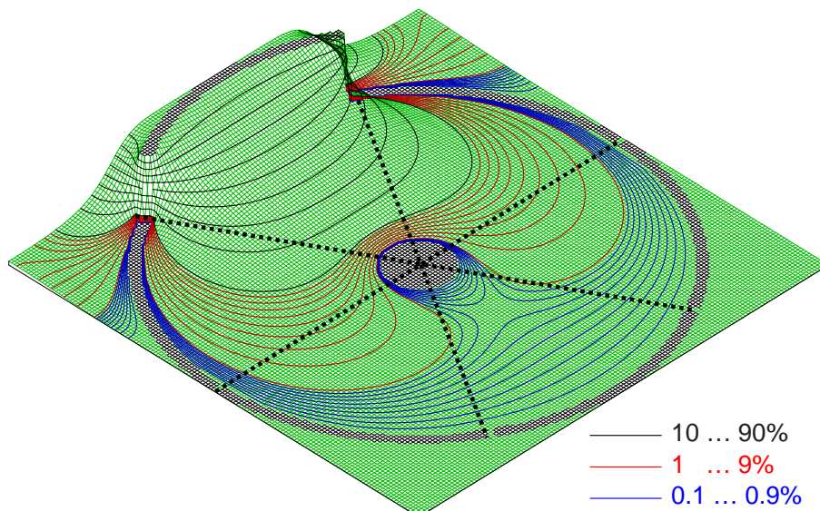
Figure 3.1: Weighting potential \psi_1 for a segment of a 6-fold segmented MINIBALL detector in the coaxial region of the detector.
