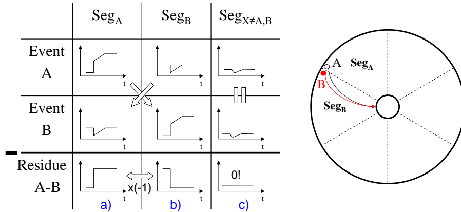
Figure 5.6: A novel method to extract derivative crosstalk in segments \text{Seg}_X is based on the charge pulses which are caused by interactions close to the segmentation line between \text{Seg}_A and \text{Seg}_B . To illustrate the procedure only schematic pulses and subtracted pulses are shown. Ideal pulses from measurements done at position A and B are subtracted. Derivative crosstalk contributions would be determined from non-vanishing pulses in segments \text{Seg}_X in row c (details see text).
