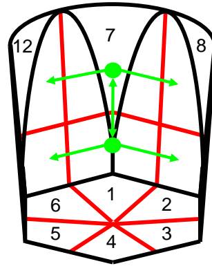
Figure 5.3: Schematic view of the crystal indicating the labeling of the 12 segments of the detector. Observed crosstalk induced by a segment is only picked up by its three closest neighbors. Two examples illustrate this behavior: a charge signal in front segment 1 induces crosstalk signals in segments 2, 6 and 7; a charge signal in back segment 7 induces crosstalk signals in segments 1, 8 and 12.
