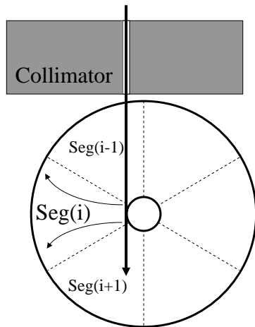
Figure 10.1: Setup of the collimator as used for creating events near the core. By gating on Seg(i), a region near the core could be selected.
