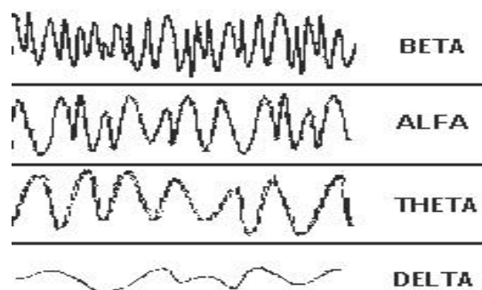
Figure 1: Brain wave samples beta, alpha, theta, and delta band.
