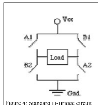
Figure 4: Standard H-Bridge circuit
