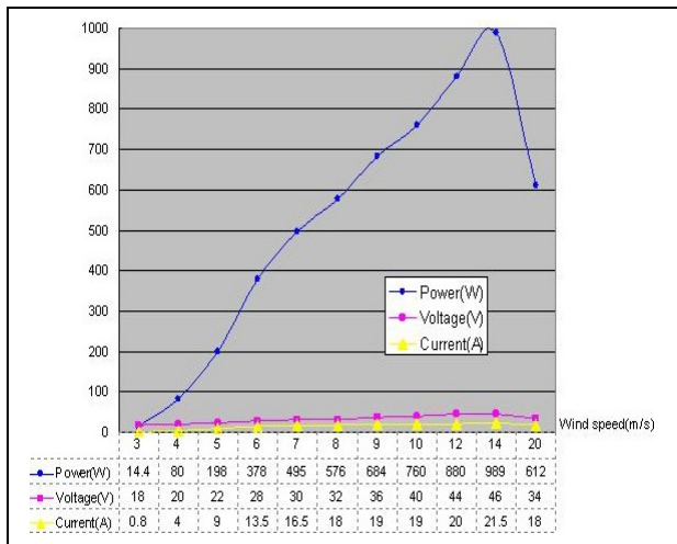
Figure 2: 500W Wind Generator Manufacturer Performance Datasheet
