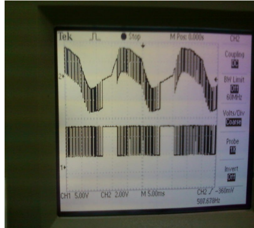
Fig.15: Voltage output of the half bridge of the H-bridge shown in channel 2 of the oscilloscope
