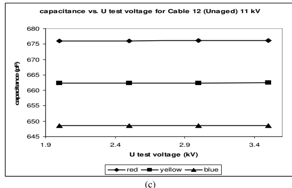
Fig. 12. Capacitance values for cables 8 (a), 9(b) and 12(c) (unaged)
