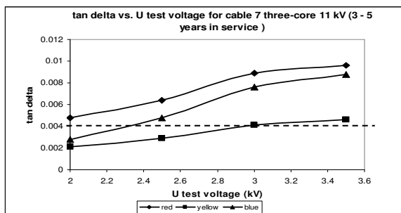
Fig. 7. Inconsistent the increasing of tan delta value for every single (red, yellow and blue) three-core cable after 3 - 5 years in service
