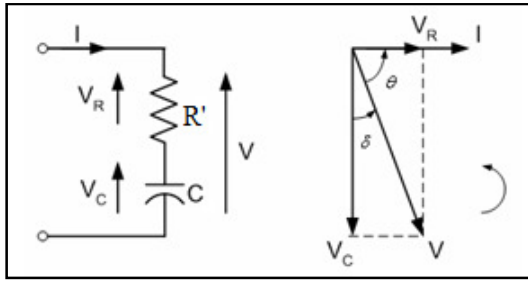
Fig. 3: Series RC model equivalent circuit and phasor diagram
