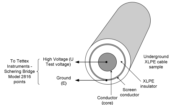
Fig. 4. Measurement setup for single-core of XLPE underground cables
