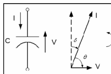
Fig. 1: Capacitor and phasor diagram, I (current) lead V (voltage) at \theta^\circ and \delta is loss angle
