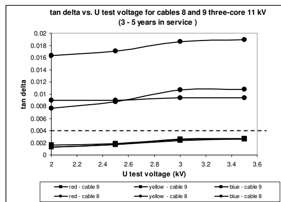
Fig. 10. The comparison of low and high values of tan delta for two three-core cables after 3 – 5 years in service
