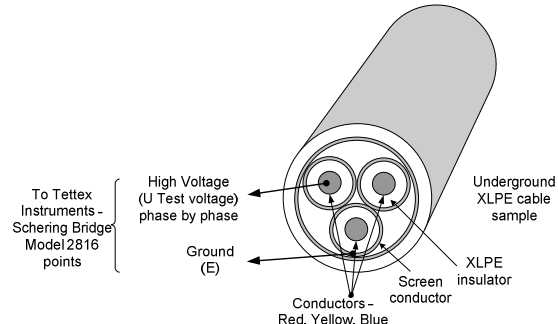
Fig. 5. Measurement setup for three-core of XLPE underground cables
