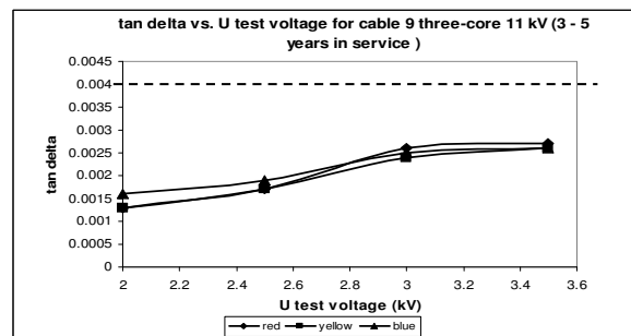
Fig. 9. The low value of tan delta for three-core cable after 3 – 5 years in service
