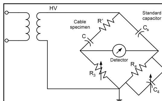
Fig. 2: Schering Bridge
