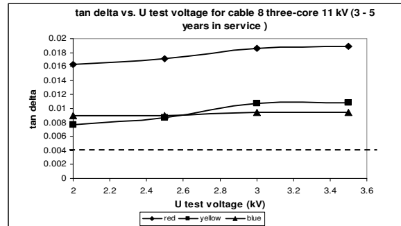
Fig. 8. The high value of tan delta for three-core cable after 3 – 5 years in service
