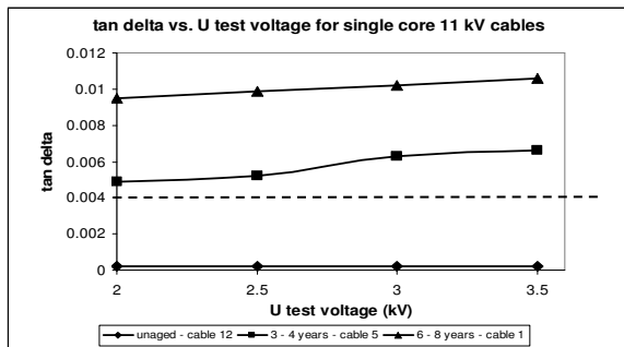
Fig. 6. Comparison of tan delta versus U test voltage after sometime in service and unaged of cables
