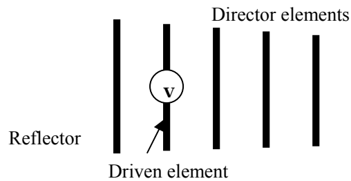
Figure 2.4. Yagi-uda configuration using dipole elements
