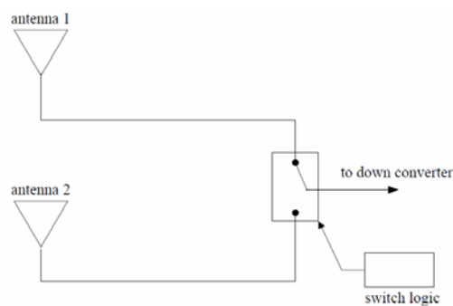
Figure 2.1. Selection combining
