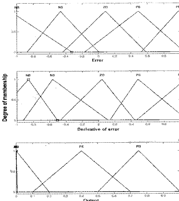
Fig.7 Optimised MFs of the fuzzy controller
