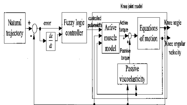
Fig.4 PD-type fuzzy control
