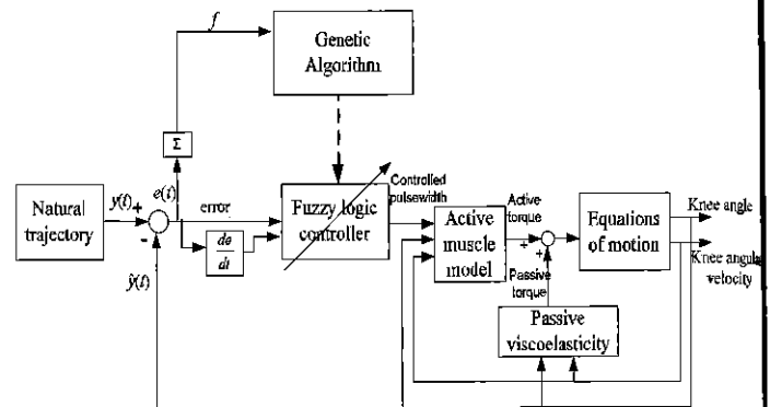
Fig. 6 GA optimization of fuzzy controller
