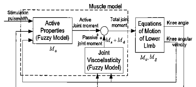
Fig. 1 Schematic representation of the knee joint model
