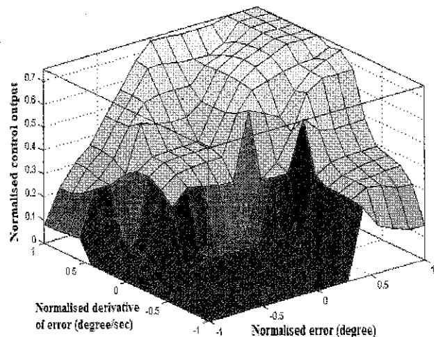
Fig. 9 Nonlinear control surfaces of the optimized FLC
