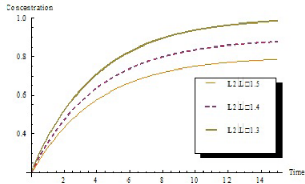
Fig. 2. Profile the concentration as a function of time of a prolate spheroidal drop for L2/L = 1.3, 1.4, and 1.5
