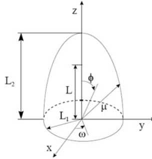
Fig1. Characteristics of a prolate spheroidal drop
