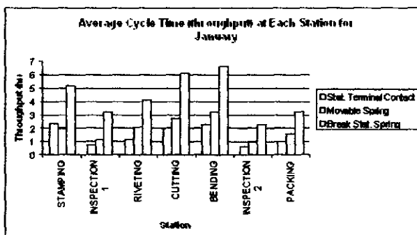
Figure 4. Average throughput time at each station, TT_j^*
