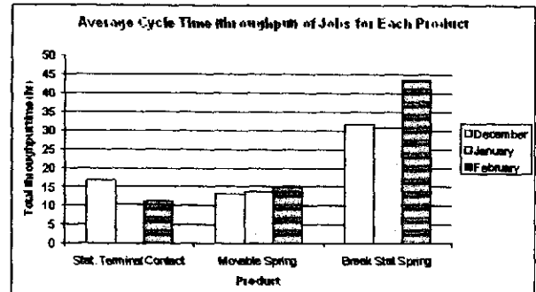
Figure 5. Average throughput time of jobs, TT_j , for each product
