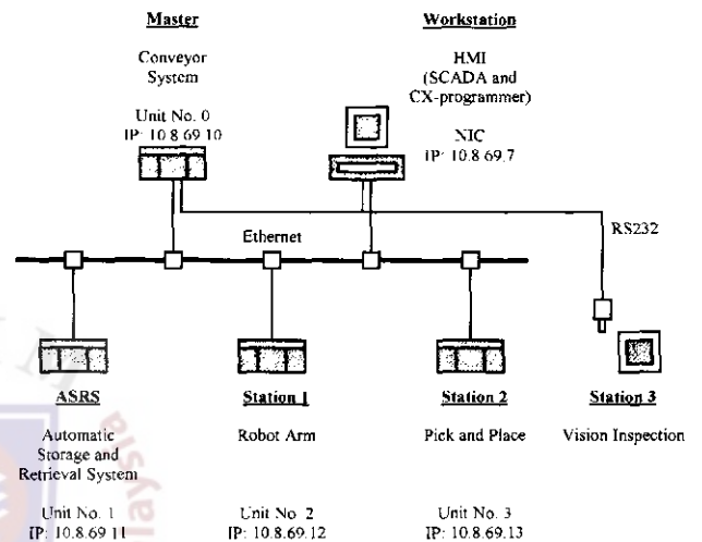
Figure 3: CIM-70E system architecture
