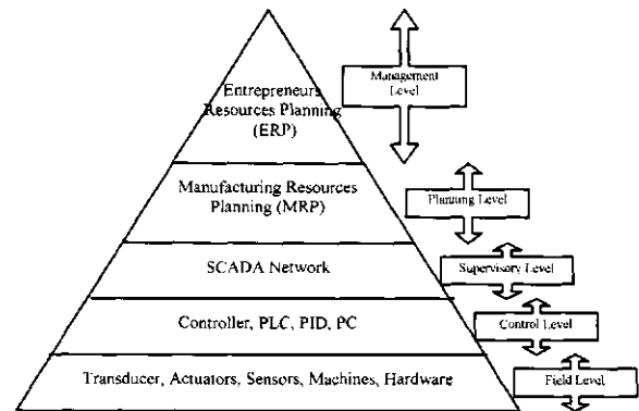
Figure 1: Pyramid of industrial automation system.
