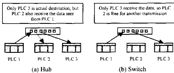
Figure 2: Ethernet network method using hub/ switch.
