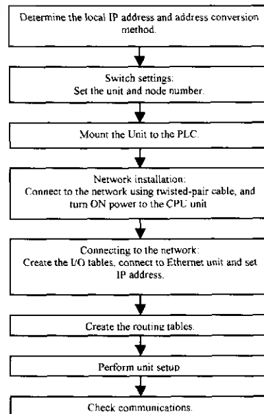
Figure 4: Overview of Ethernet unit installation procedure
