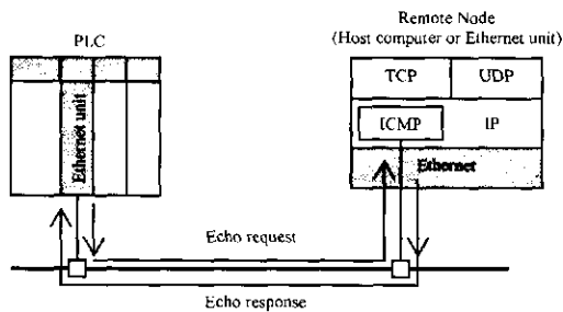
Figure 5: PING command [8]
