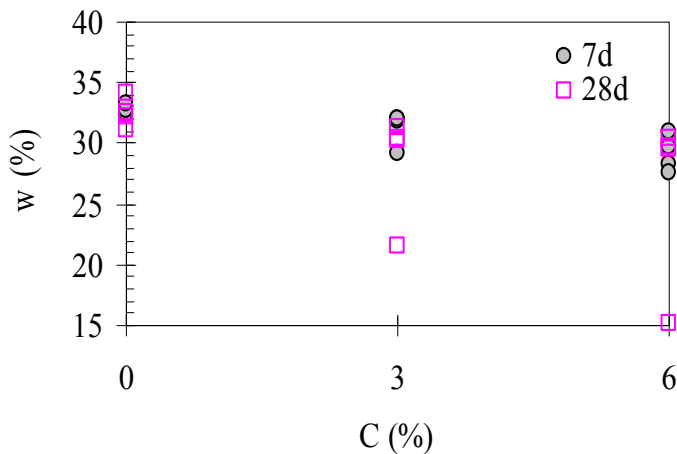
Fig. 2: Water content – cement content
