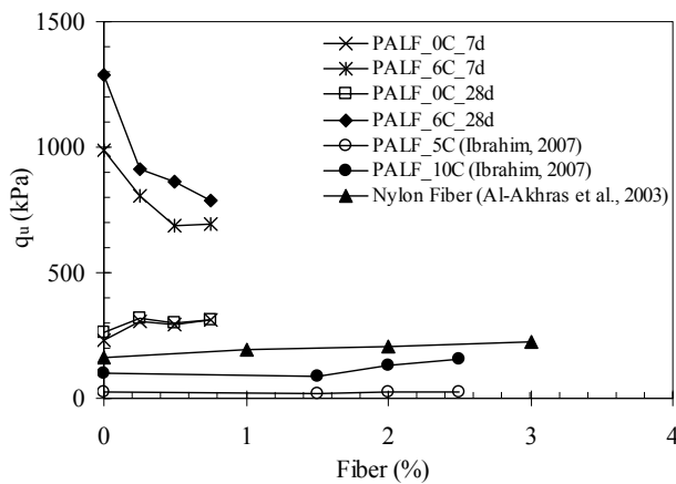
Fig. 7: Comparison of q_u for fibre-treated soils
