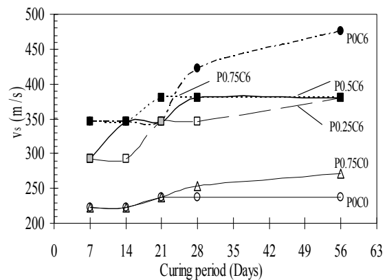
Fig. 4: S-wave velocity-curing period.
