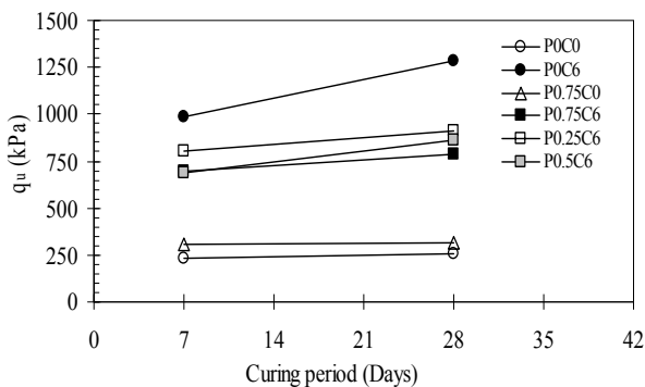
Fig. 5: Unconfined compressive strength – curing period.
