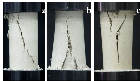
P0.25C3 P0.75C6 P0.75C0 Fig. 8: Typical failure modes of UCS test specimens
