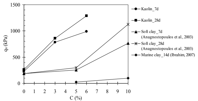
Fig. 6: Comparison of q_u for cement treated soils
