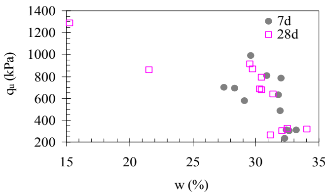
Fig. 3: q_u ( kPa ) – w (%).
