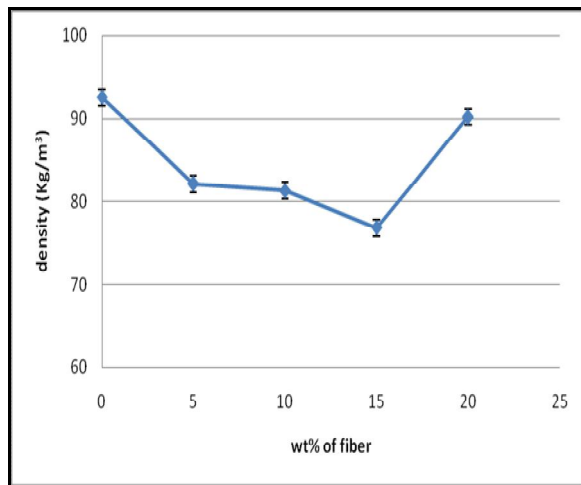
Fig. 7. Density of pu/coir at different fiber wt%
