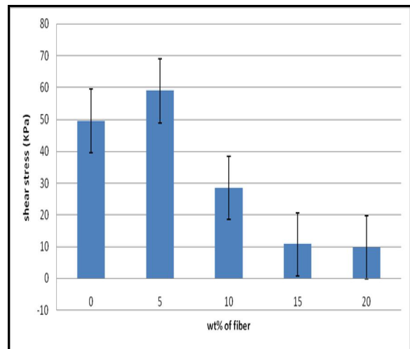
Fig. 9. Shear stress of pu/coir panel at different fiber wt%
