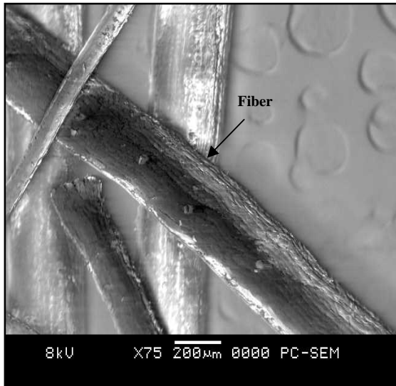
Fig 4. Untreated coir fiber surface at 75X magnification
