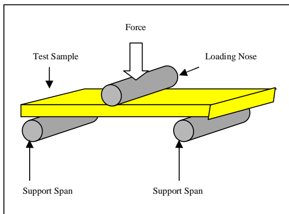
Fig. 3. Three point bending testing schematic diagram
