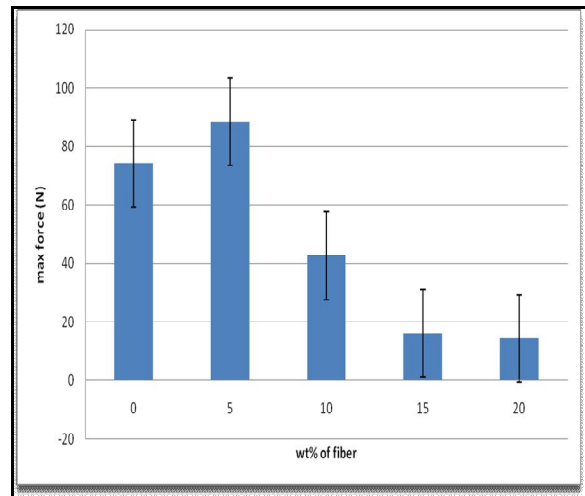
Fig. 8. Maximum force of pu/coir panel at different fiber wt%
