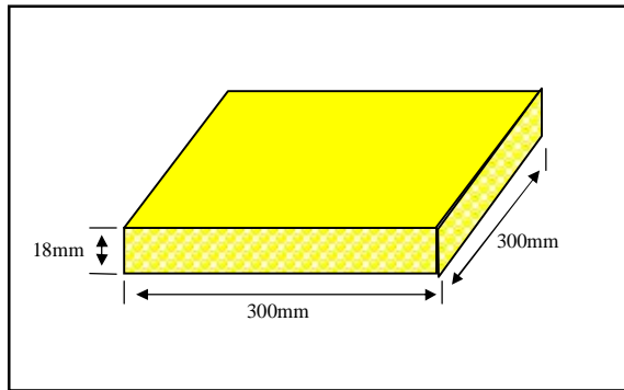
Fig. 2. Dimension of density test sample
