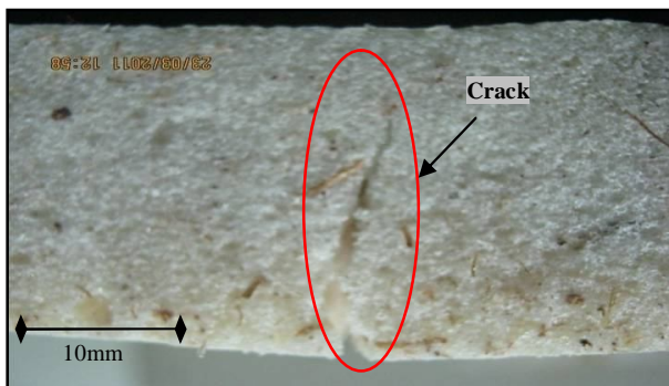
Fig. 11. Tensile failure on composite foam panel
