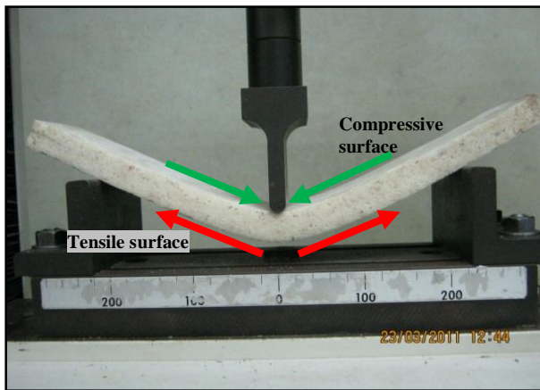
Fig 10. Testing sample at failure
