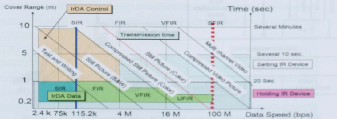
Figure 1.3 Infrared transmission speed, time and coverage area [1.23]
