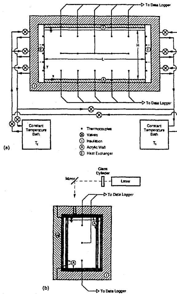
Figure 2.1 Schematic diagram of the test cell in [20]: (a) front view; (b) end view.
