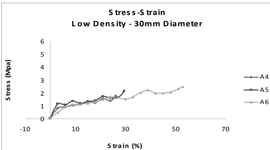
Figure 7. Compressive Stress-Strains curve
