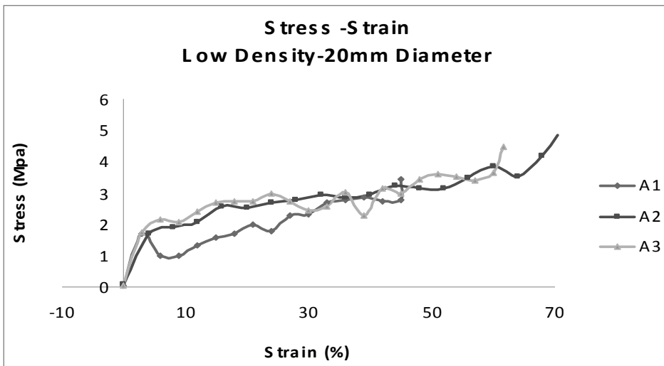
Figure 6. Compressive Stress-Strains curve
