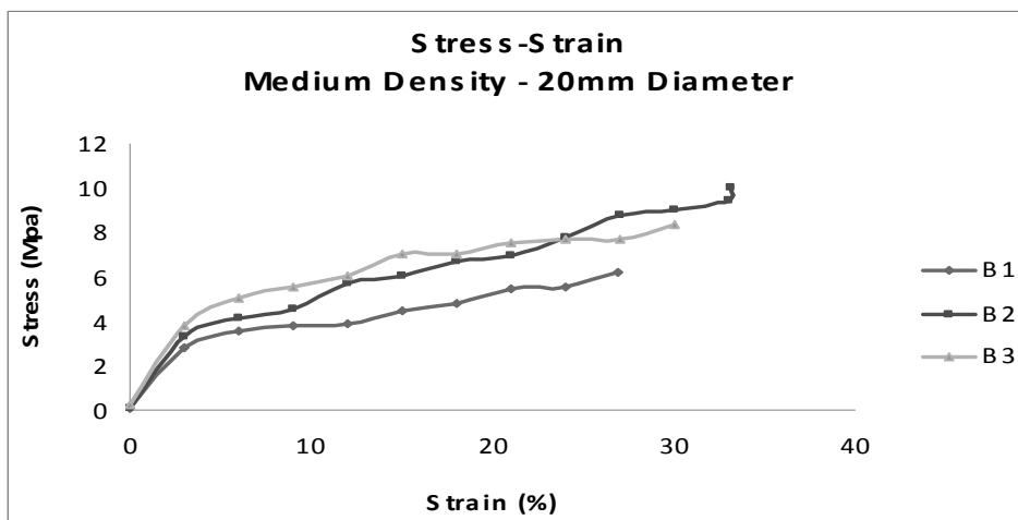
Figure 10. Compressive Stress-Strains curve
