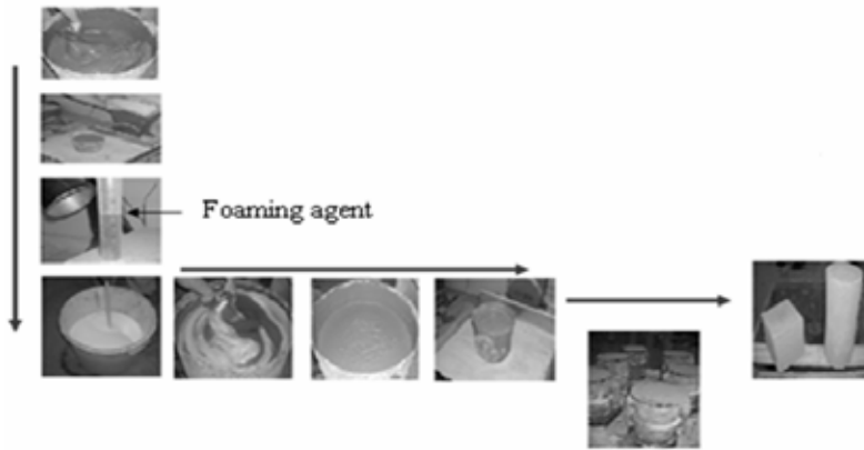
Figure 1. Manufacturing of foamed concrete
