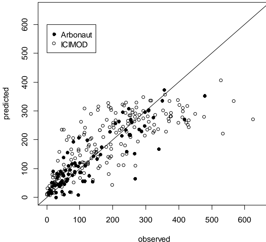
Figure 6. Lidar estimated AGB (T ha-1) using the previously mentioned variables (Table 1) plotted against field measured AGB for Arbonaut and ICIMOD AGB models.
