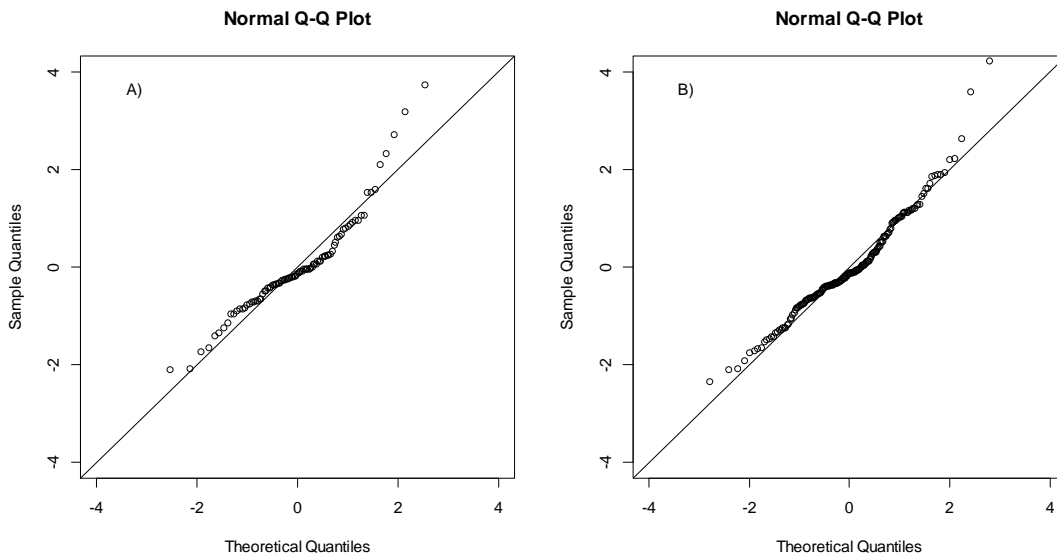
Figure 9. QQ plot of the residuals for Arbonaut (A) and ICIMOD (B) models. The graph shows that neither one of the models produced residuals that are normally distributed.
