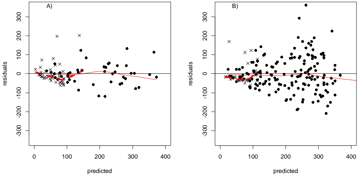
Figure 11. AGB residuals plotted against the predicted values for Arbonaut (A) and ICIMOD (B) AGB models and for strata 1 (dots) and strata 2 (crosses) representing respectively dense and sparse forests. The red continuous line represents the locally-weighted polynomial regression for the strata 1 while the dashed line represents the locally-weighted polynomial regression for the strata 2 (lowess function, R project).
