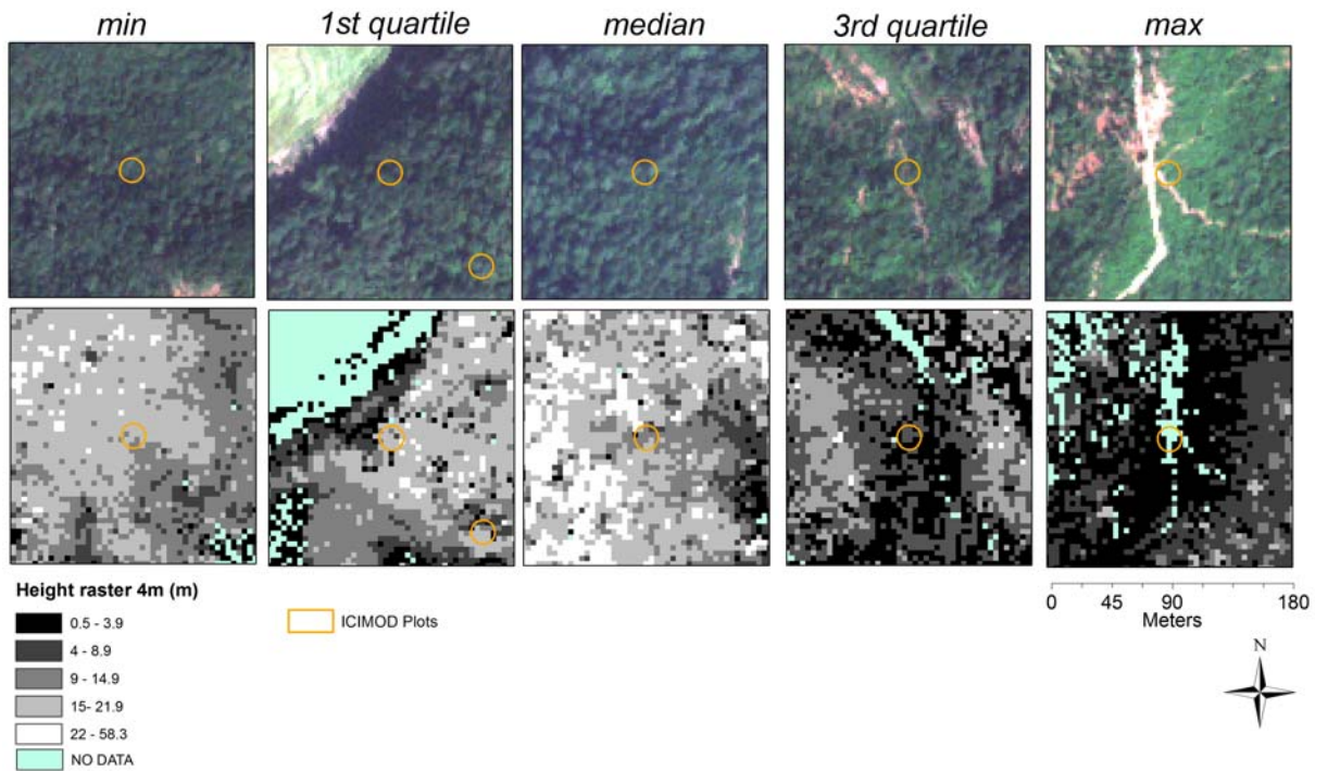
Figure 5. Range (minimum, 1 st quartile, median, 3 rd quartile, maximum values) of height Coefficient of Variation (CV) for the ICMOD plots. No data values are pixels where there is no vegetation laser hit.
