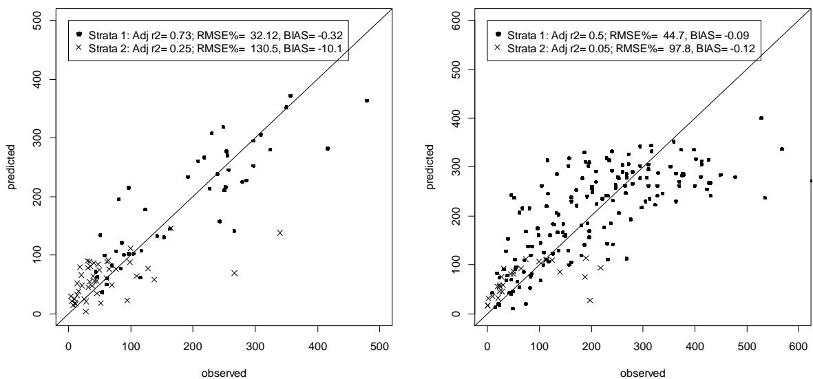
Figure 10. Lidar estimated AGB (T ha-1) plotted against field measured AGB for Arbonaut and ICIMOD AGB stratified models.
