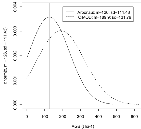
Figure 13. Above Ground Biomass ( t\ ha^{-1} ) density distribution function for the Arbonaut and ICIMOD datasets. The vertical lines show the mean values.
