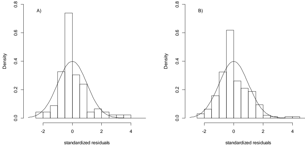
Figure 8. Standardized AGB residuals frequency distribution for Arbonaut (A) and ICIMOD (B) models.
