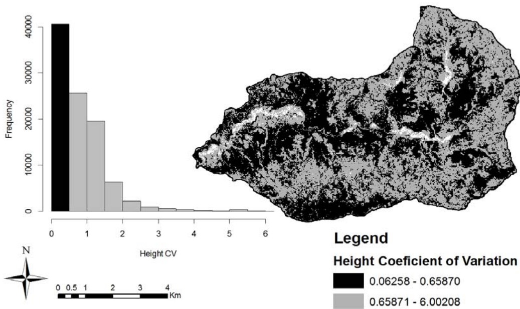
Figure 3. Frequency and geographical distribution of the Height Coefficient of Variation (HCV) within the Ludikhola watershed. The two strata are defined by the median HCV value (0.6587), in black the first strata representing the denser and uniform forests, while in grey are the more sparse forests and trees outside forests.
