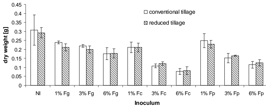
Figure 5. First bioassay. Shoot dry weight of wheat plants (mean±SD, n=3 ). In non-infested soil (NI) and soils infested at 1%, 3%, 6% with F. graminearum (Fg), F. culmorum (Fc) or F. pseudograminearum (Fp).
