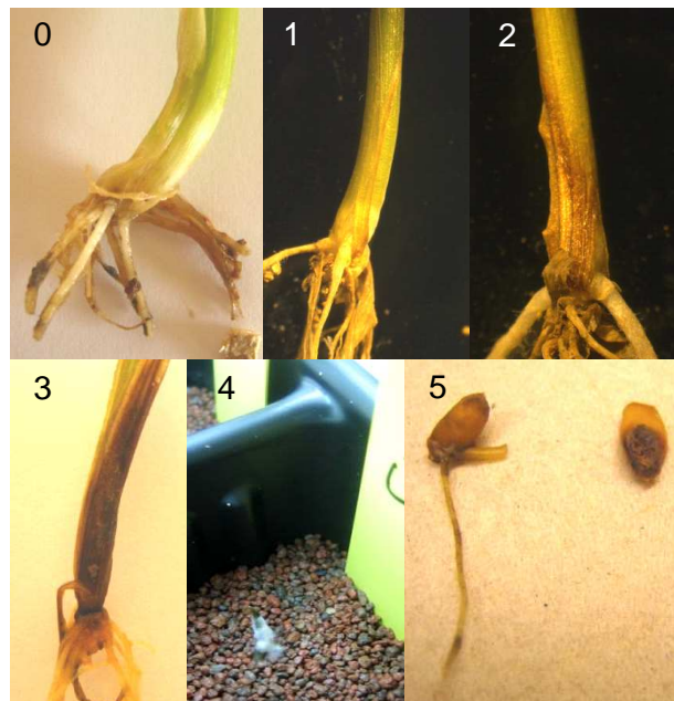
Figure 2. Disease scoring of wheat plants showing symptoms of fusarium foot rot. Step 0-5.
