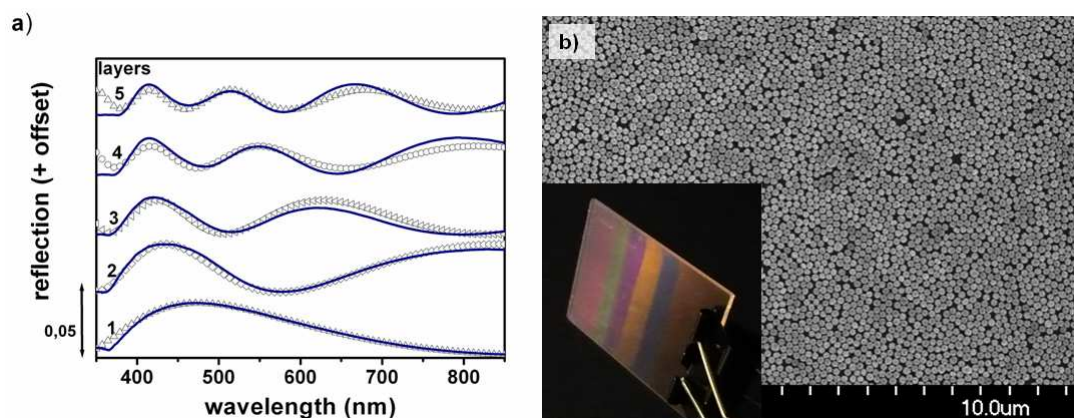
Fig. 4. a) Measures and calculated reflectance spectra of 234\pm 11 nm ZnO particles. b) SEM image of the single layered Langmuir-Blodgett film, the inserted photograph shows the different colours of the 1-5 layered film in reflection.
