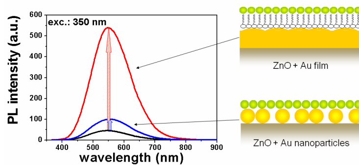
Fig. 2. Photoluminescence emission enhancement due to plasmonic interactions in Au-ZnO hybrid films.
