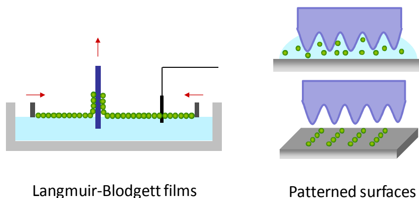
Fig. 1. 2D particle assembly techniques used in this thesis.
