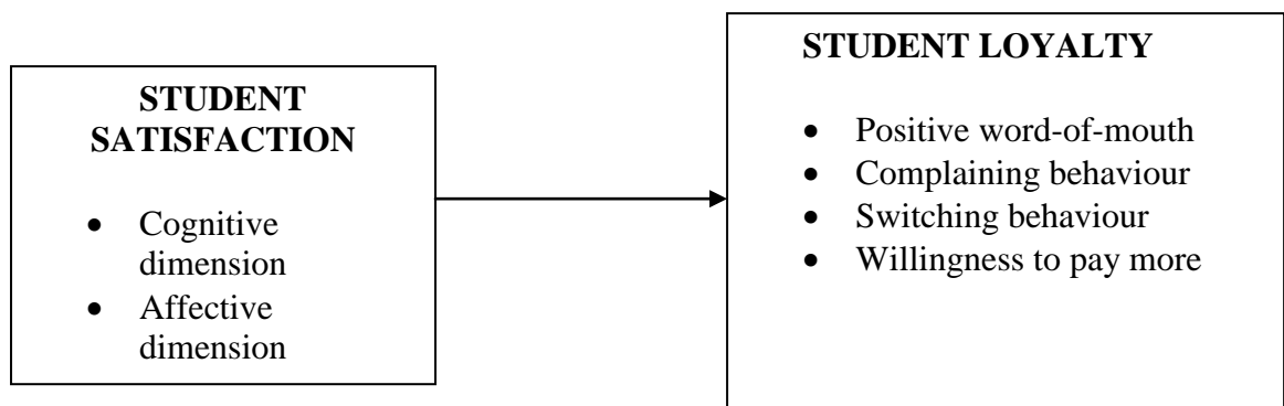
Figure 2.1 Theoretical framework
