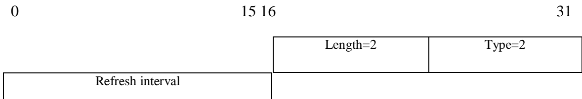
Figure 2.11: Binding Refresh Advice option
