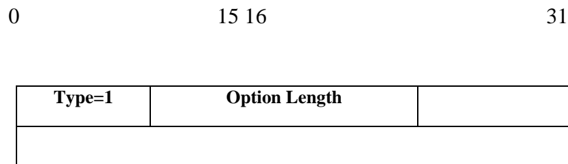
Figure 2.10: PadN option
