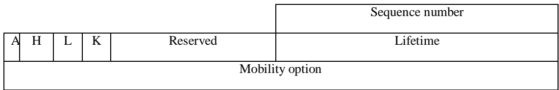
Figure 2.5: Binding Update message
