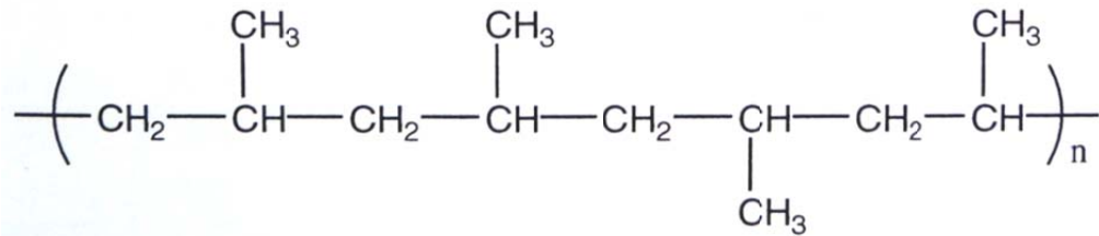
atactic polypropylene
