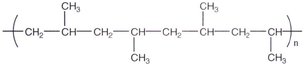
syndiotactic polypropylene
