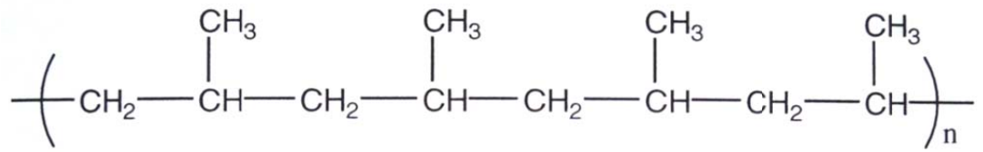
isotactic polypropylene
