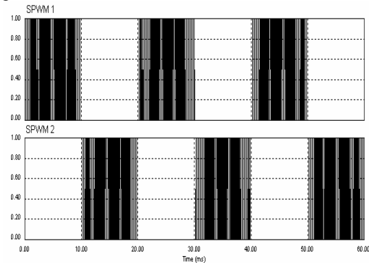
Figure 5 - Simulation result of SPWM 1 and SPWM 2
