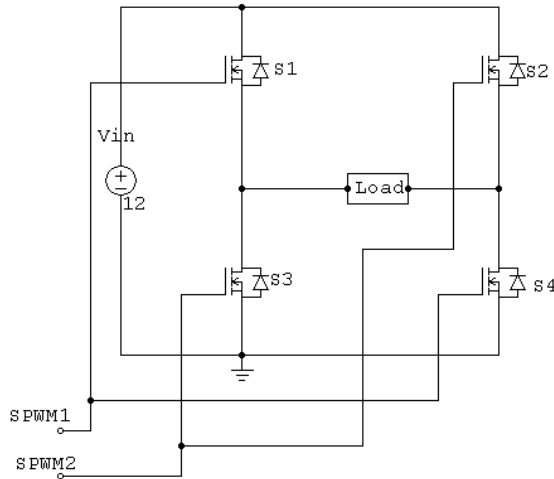
Figure 4 - Switching strategy for Single Phase Inverter
