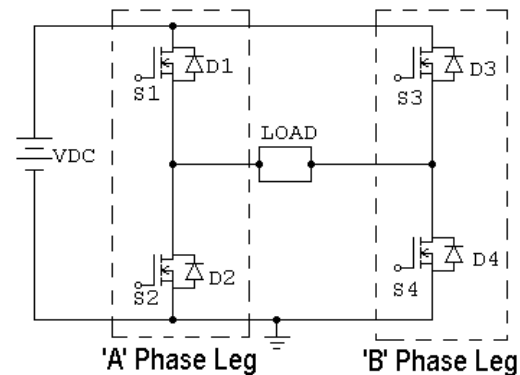
Figure 2 - Full Bridge Single Phase Inverter
