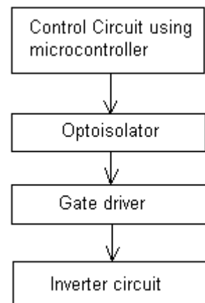
Figure 3 - Flow of Hardware Development
