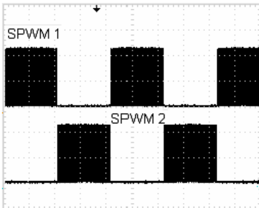
Figure 7 - SPWM 1 and SPWM 2 from port 1.7 and port 1.6 microcontrollers
