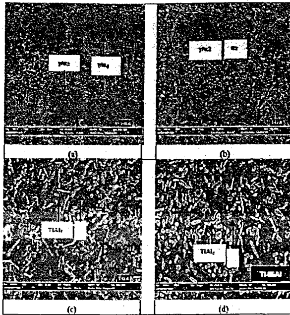
Fig.3. SEM image showing microstructure of: (a) Ti-50Al; (b) Ti-53Al; (c) Ti-60Al; (d) Ti-65Al alloy
