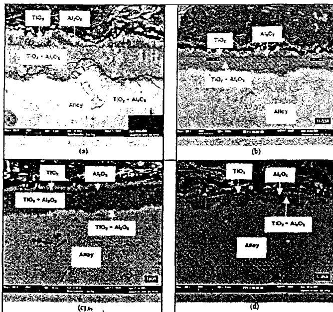
Fig.5. Cross-sectional microstructures after oxidation in air at 1173K for 50 hours of : a) Ti-50Al; b) Ti-53Al; c) Ti-60Al and d) Ti-65Al alloy
