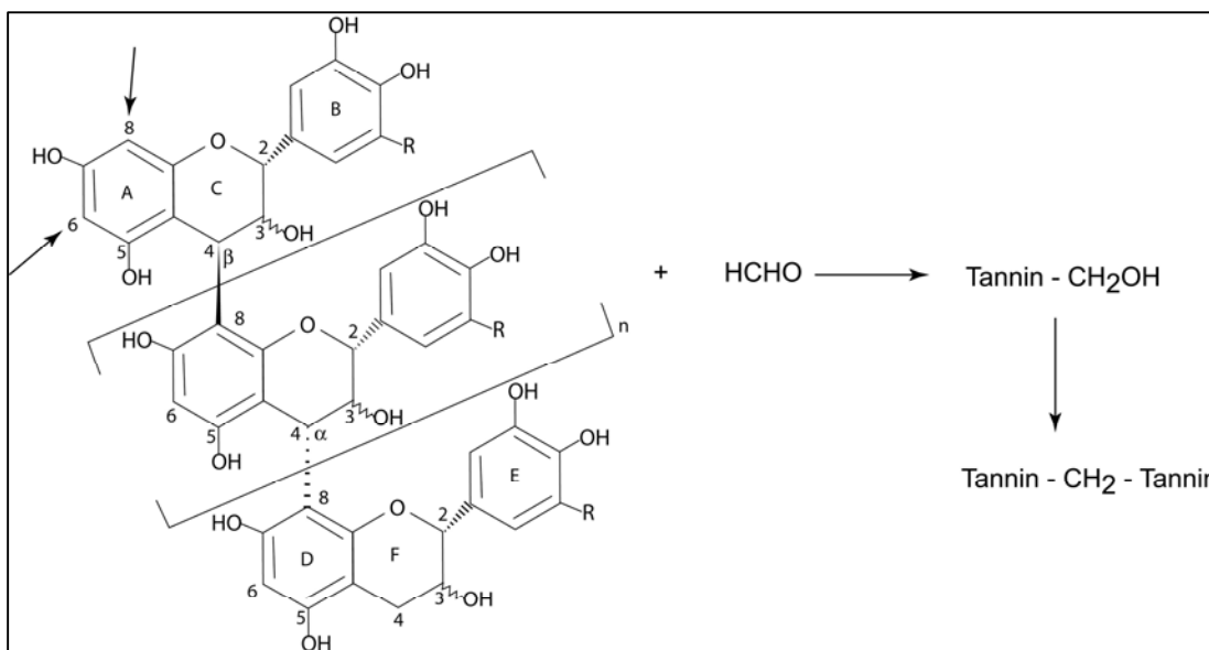
Fig. 1.7 Reaction of tannins with formaldehyde (arrow pointed are the reactive sites of tannins with formaldehyde) (Pizzi, 1983b).
