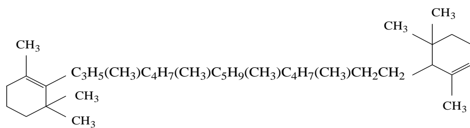
\alpha - carotene
