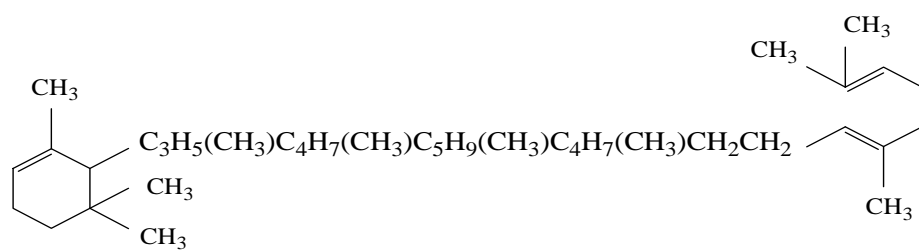
\delta - carotene
