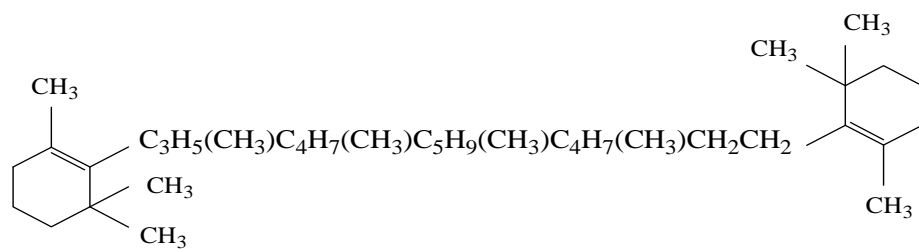
\beta - carotene
