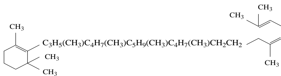
\gamma - carotene
