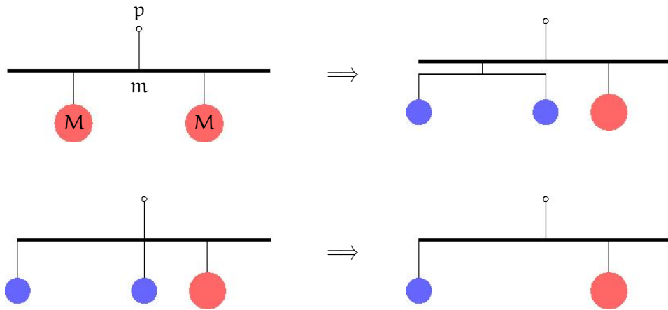
Figure 1: The law of the lever ‘derived’ from alleged symmetry considerations. The step from the upper right (second) to the lower left (third) picture does not follow. The small (blue) balls represent half the mass of the big (red) balls.
