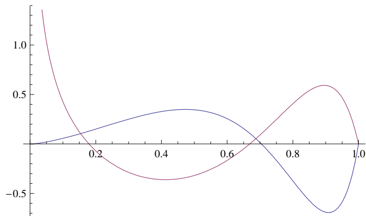
Figure 8.7: Two-dimensional plot of the weight function \tau(z) = \omega(z) . The first branch cuts the horizontal z -axis at the points z = 0, 0.7, 1 , and it never touches the vertical axis, whereas the second branch cuts the z -axis at z = 0.18, 0.67, 1 , and it reaches a vertical asymptote at z = 0.05 . The two branches intersect each other at z = 0.15, 0.69, 1 , where \tau(z) becomes single-valued.
