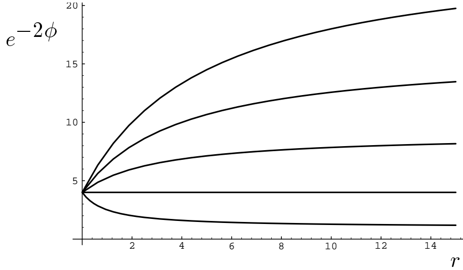
Figure 3.1: Realization of the Attractor Mechanism in the \mathcal{N} = 2 , d = 4 extremal \frac{1}{2} -BPS dilatonic BH. Independently of the set of initial (asymptotical r \rightarrow \infty ) moduli configurations (corresponding to the initial data of the dynamical flow inside the moduli space), the “near-Horizon” ( r \rightarrow 0^+ , with r denoting the radial distance from the Event Horizon) evolution of the moduli-dependent dilatonic function g^{-2}(\phi) \equiv e^{-2\phi} converges towards a fixed “attractor” value, which is purely dependent on the (ratio of the) quantized conserved charges of the BH. Such a purely charge-dependent phenomenon of “attraction” of the moduli field configurations encodes the intrinsic loss of information in the (equilibrium) thermodynamics of the extremal dilatonic BH.
