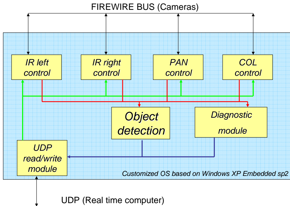
Figure 7 - Image processing software architecture
