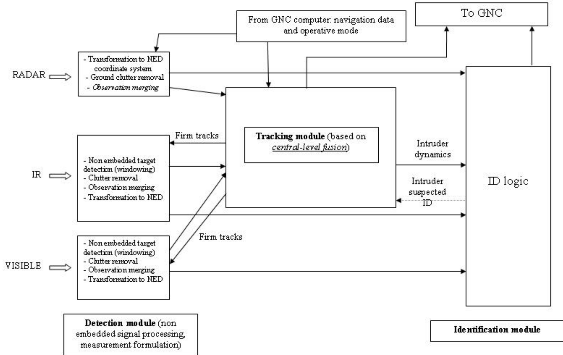
Figure 10 – Sensor fusion logical architecture
