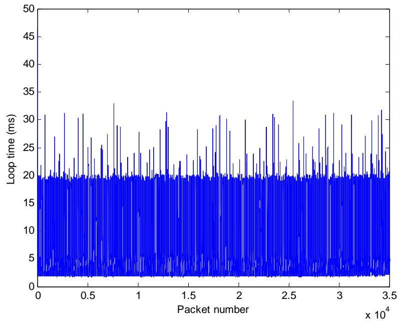
Figure 15 – Loop time for all the CAN packets with introduction of an inter-message time of 280 \mu\text{s}
