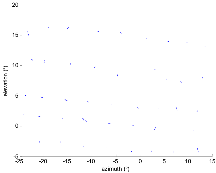
Figure 20 - Vector representation of azimuth and elevation differences (color camera, 2 nd session)
