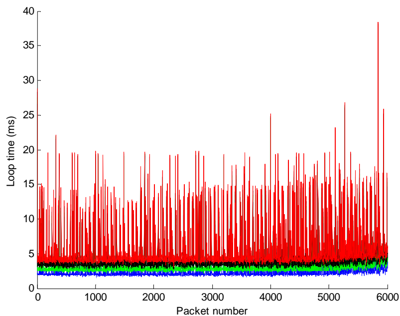
Figure 16 – Loop time for messages with different priority with introduction of an inter-message time of 280 \mu\text{s}
