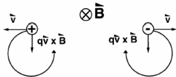
Fig. 4a-Lorentz force on a charged particle.
