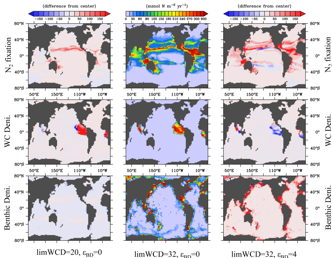
Fig. 2. Global distribution of annual vertically integrated \text{N}_2 fixation (top row), water column denitrification (middle row) and benthic denitrification (bottom row) for the experiments \text{limWCD} = 20 , \varepsilon_{\text{BD}} = 0 (left); \text{limWCD} = 32 , \varepsilon_{\text{BD}} = 0 (center); and \text{limWCD} = 32 , \varepsilon_{\text{BD}} = 4 (right). See text for model experiment details.
