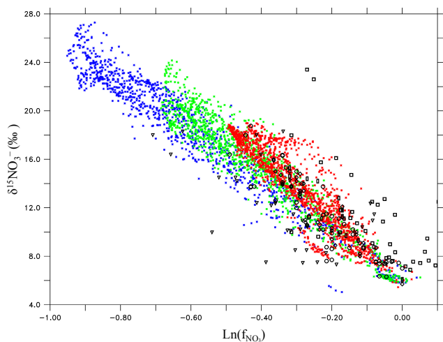
Fig. 5. Annual mean \delta^{15}\text{NO}_3^- versus expected nitrate ( f_{\text{NO}_3} ) shows the increase of \delta^{15}\text{NO}_3^- as \text{NO}_3^- is consumed in suboxic zones ( \text{O}_2 < 10 \mu\text{M} ) from the isotope effect of water column N-loss in \text{limWCD} = 20 (blue), \text{limWCD} = 26 (green), \text{limWCD} = 32 (red) and observations (black) from Cline and Kaplan (1975) ( \square ), Altabet et al. (1995) ( \Delta ), Brandes et al. (1998) ( \diamond ), Voss et al. (2001) ( \circ ), and Somes et al. (2010b) ( \square ). Note \varepsilon_{\text{BD}} = 0\text{‰} for the model experiments shown here. Expected nitrate is determined to be at the elemental ratio 15 \cdot \text{PO}_4^{3-} in the model based on experiments where WCD was switched off (not shown), which is in agreement with the expected nitrate calculation from Voss et al. (2001) based on nitrate-density isopycnals. Observations near the seafloor are excluded to avoid any impact from benthic denitrification.
