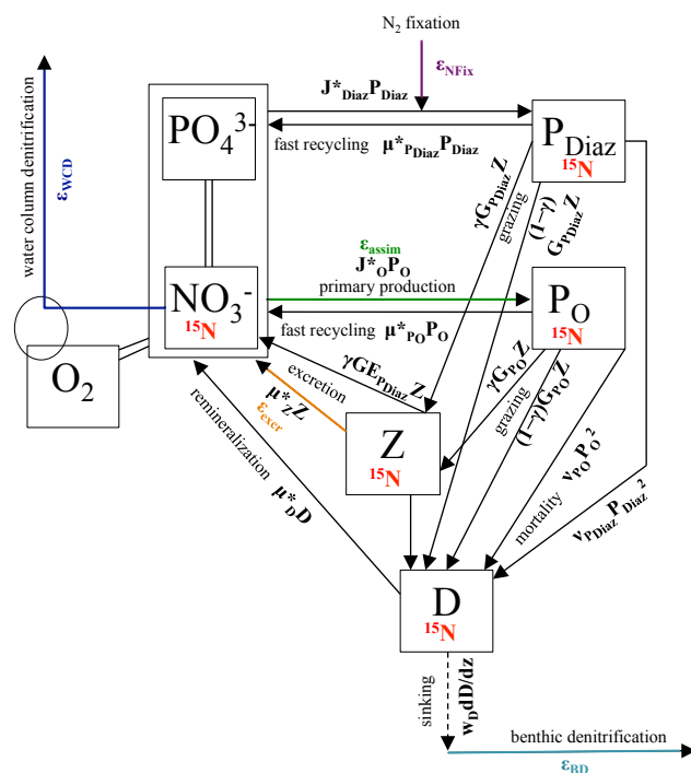
Fig. 1. Schematic of the marine ecosystem/biogeochemical model compartments including the nitrogen isotope parameters (colors) (Somes et al., 2010b). The prognostic variables include 2 nutrients, nitrate ( \text{NO}_3^- ) and phosphate ( \text{PO}_4^{3-} ), 2 phytoplankton, \text{N}_2 -fixing diazotrophs ( \text{P}_{\text{Diaz}} ) and other \text{NO}_3^- -assimilating phytoplankton ( \text{P}_O ), as well as zooplankton (Z), sinking detritus (D), and dissolved oxygen ( \text{O}_2 ).
