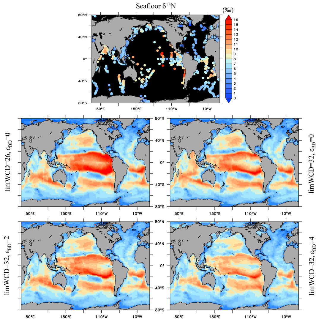
Fig. 3. Seafloor \delta^{15}\text{N} (Tesdal et al., 2012) comparison with model seafloor \delta^{15}\text{N} with \text{limWCD} = 26 , \epsilon_{\text{BD}} = 0 ; and \text{limWCD} = 32 , \epsilon_{\text{BD}} = 0 , 2, and 4‰ for all experiments shown here. Note a simple diagenetic model was applied to model sinking \delta^{15}\text{N} to account for diagenetic alteration during burial into the seafloor sediments based on seafloor depth (Robinson et al., 2012). See text for additional details.
