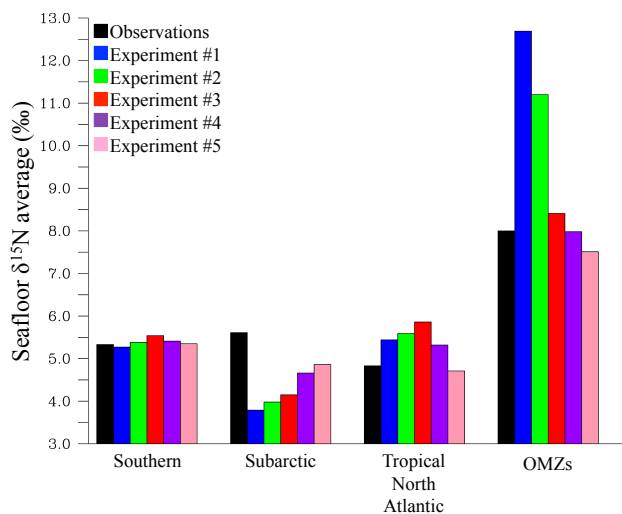
Fig. 4. Comparison of average seafloor \delta^{15}\text{N} in the Southern Ocean ( 50\text{--}75^\circ\text{S} ), subarctic/Arctic Ocean ( 50\text{--}75^\circ\text{N} ), tropical North Atlantic ( 0\text{--}25^\circ\text{N} ), and oxygen minimum zones ( \text{O}_2 < 10\text{ }\mu\text{M} ) with observational values in parentheses. Note we include locations of observed and simulated OMZs to account for the displaced model OMZs in this comparison.
