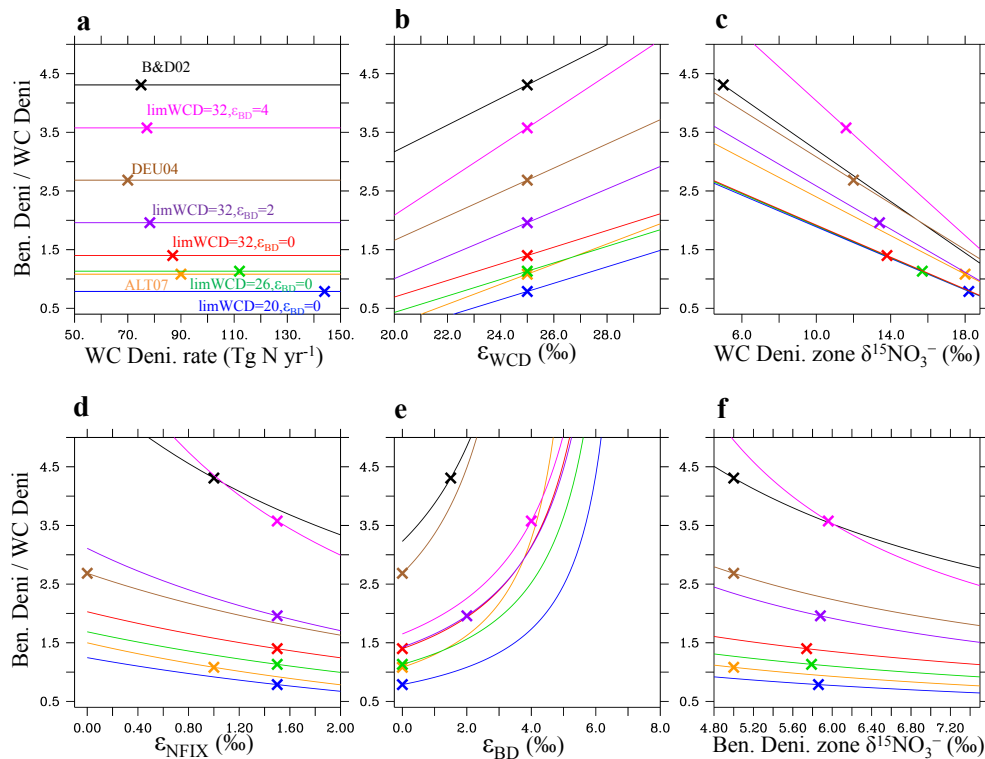
Fig. 6. Results of the one-box \delta^{15}\text{NO}_3^- model with different nitrogen isotope parameter settings according to previous configurations (Brandes and Devol, 2002; Deutsch et al., 2004; Altabet, 2007) and this study (Table 4). Each panel shows the sensitivity of one parameter on the ratio of benthic denitrification to water column denitrification (BD : WCD) needed to achieve observed global mean \delta^{15}\text{NO}_3^- in a steady-state scenario while all other parameters are held constant: (a) WCD rate, (b) WCD fractionation factor ( \epsilon_{\text{WCD}} ), (c) average \delta^{15}\text{NO}_3^- value where WCD occurs, (d) \text{N}_2 fixation fractionation factor ( \epsilon_{\text{NFIX}} ), (e) benthic denitrification fractionation factor ( \epsilon_{\text{BD}} ), and (f) average \delta^{15}\text{NO}_3^- value where benthic denitrification occurs. Note \epsilon_{\text{NFIX}} makes diazotroph biomass depleted in \delta^{15}\text{N} by its associated value. The crosses (X) show the parameter chosen for each reported model configuration and denotes the BD to WCD ratio of the previous studies as well as coupled three-dimensional experiments from this study.
