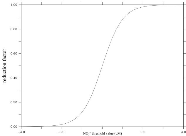
Fig. B1. Reduction factor applied to water column denitrification for given \text{NO}_3^- concentration ( \mu\text{M} ) thresholds.
