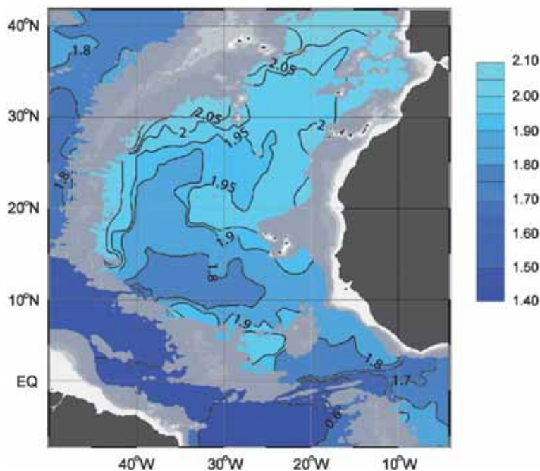
Fig. 5. Distribution of potential temperature ( ^{\circ}\text{C} ) at the bottom in the eastern part of the North Atlantic based on the WODB-2009 data. The data below 4000\text{ m} is presented. Gray shade shows the bottom topography above 4\text{ km}
