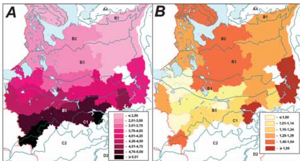
Fig. 5. A – 2046–2065 forecasted average growth of timber (m 3 /ha). B – Forecasted “shifts” of the average values of growth of timber in comparison with the period of “the modern climate” (only for “forest” regions of the EPR). Explanations are in the text.
