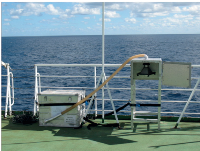
Fig. 8.2: The HVAS, "frequent flyer," installed on the monkey deck
