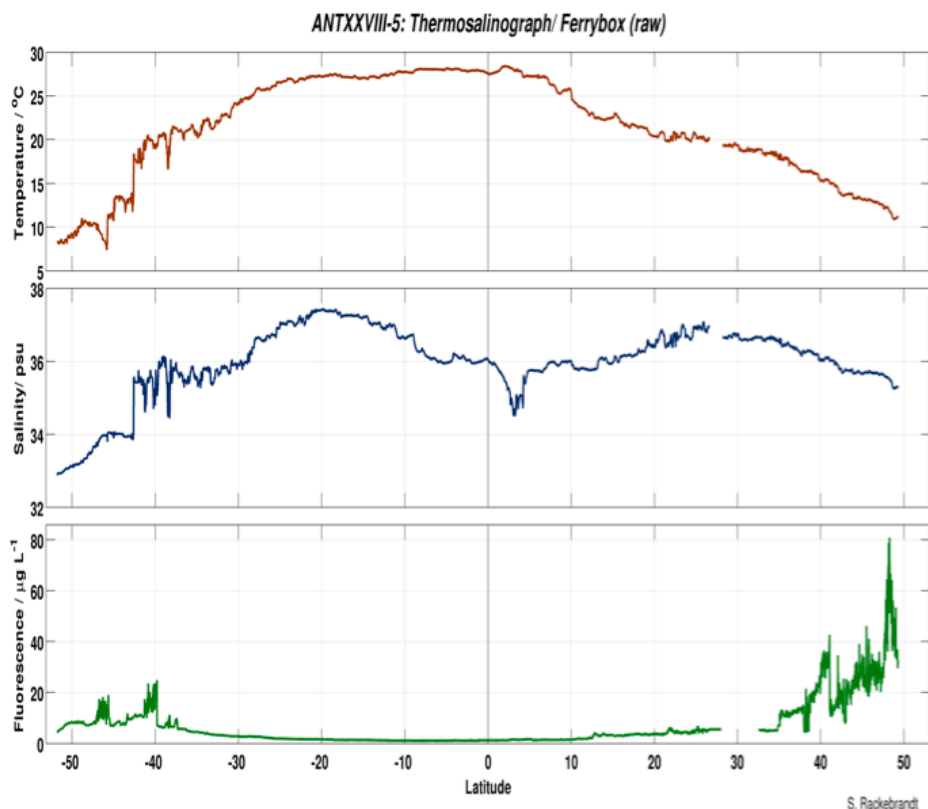
Fig. 6.2: Uncalibrated sea surface temperature, salinity and chlorophyll fluorescence between 52 °S and 49 °N in the Atlantic as measured by the ships's salinometer and ferry box
