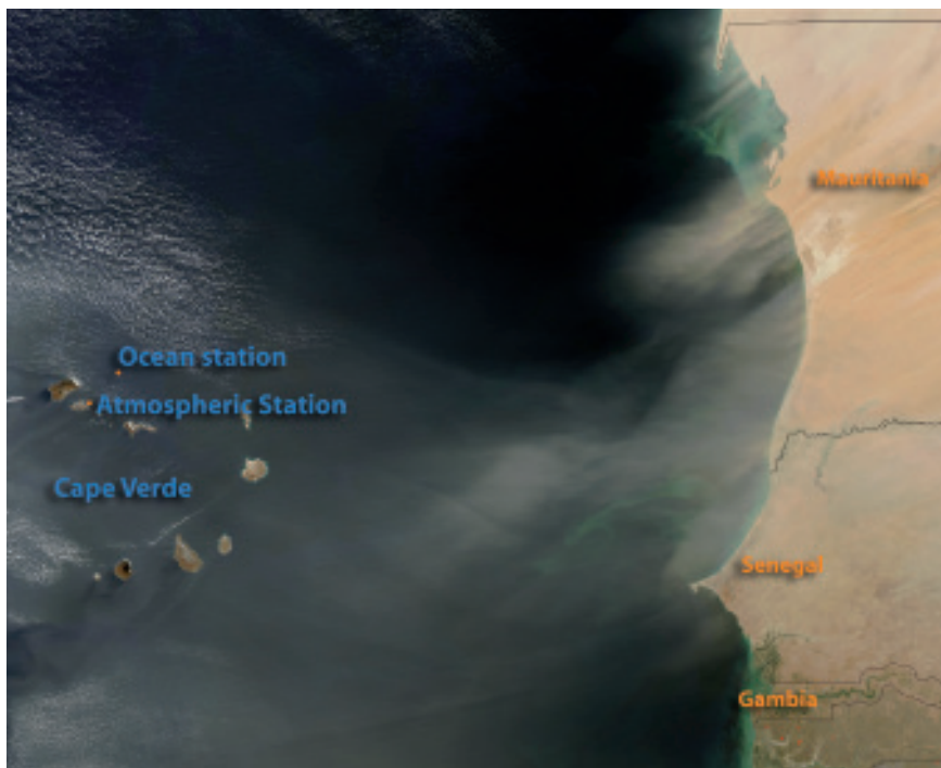
Satellite image showing a dust storm from the Sahara desert approaching the Cape Verde Islands. Image source: Visible Earth, MODIS Rapid Response Team.
