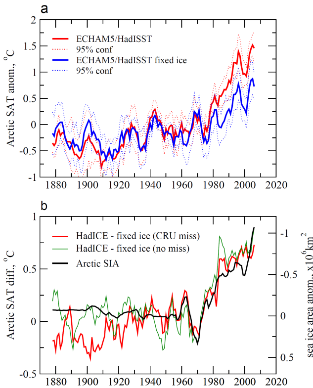
Fig. 4. (a) Arctic land SAT cold season anomalies ( ^{\circ}\text{C} ) as simulated in the HadISST (red) and HadISST-fixed ice ensemble (blue). The ensemble means are given as solid bold lines, the confidence intervals as thin dashed lines; (b) difference between the ensemble mean SATs shown in (a) with (red) and without (green) data sampling according to CRUTEM3 data. The black line depicts the inverted (see right y-axis) sea ice area differences ( 10^6 \text{ km}^2 ) (HadISST1.1 – climatology of the period 1941–1950). All time series are smoothed with a 5-yr running mean filter.
