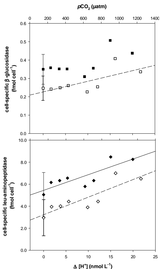
Fig. 10. Relationships between seawater p\text{CO}_2/\Delta proton concentration ( \Delta [H + ]) and cell-specific extracellular enzyme activities. Separate correlations are shown for rates integrated over days 4–20 (open symbols) and the whole experiment (filled symbols). Lines represent significant ( p < 0.05 ) linear regressions ( \beta -glucosidase, d 4–20: r^2 = 0.53 ; leu-aminopeptidase, d 4–20: r^2 = 0.79 , whole experiment: r^2 = 0.57 ).
