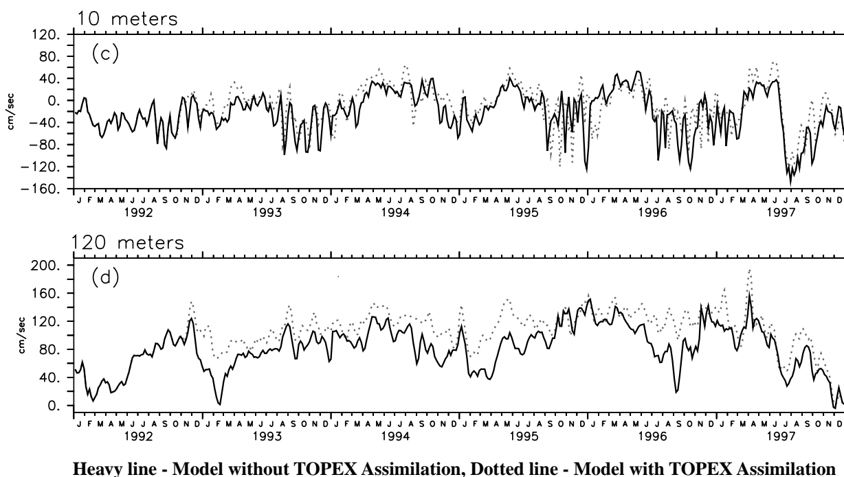
Figure 1: Model - observations comparisons at 140°W (upper) and impact of TOPEX at 140°W (lower)
