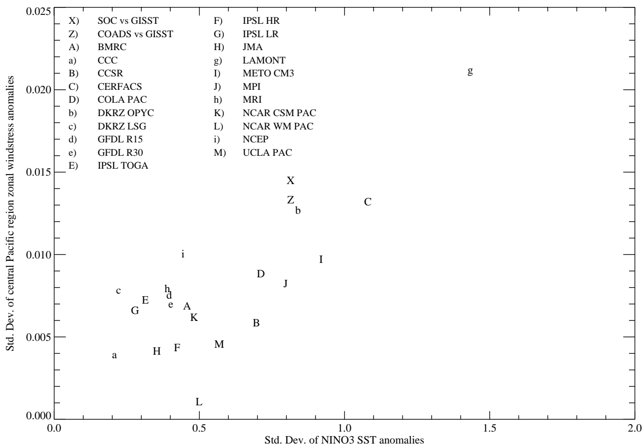
Fig. 2: Scatterplot of interannual standard deviations of SST in region Niño-3 and zonal wind stress in the central equatorial Pacific (5N-5S,165E-225E). Lower case symbols indicate models with flux adjustment, while X and Z indicate observed values.
