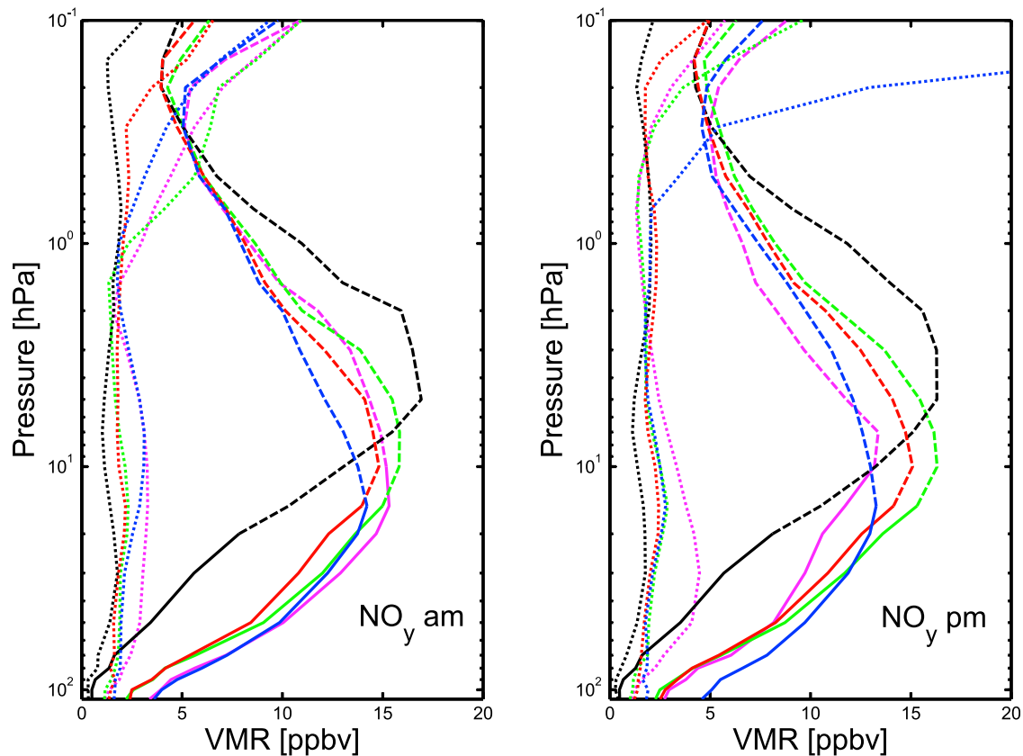
Figure 8. Same as Figure 7 but for NO y * . Dashed lines indicate where scaled initial guess values contribute to the median value. Dotted lines indicate the 1 standard deviation spread of data in each latitude bin.
