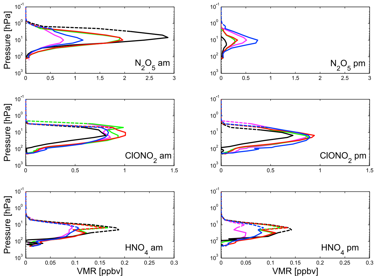
Figure 7b. Same as Figure 7a but for \text{N}_2\text{O}_5 , \text{ClONO}_2 , and \text{HNO}_4 .
