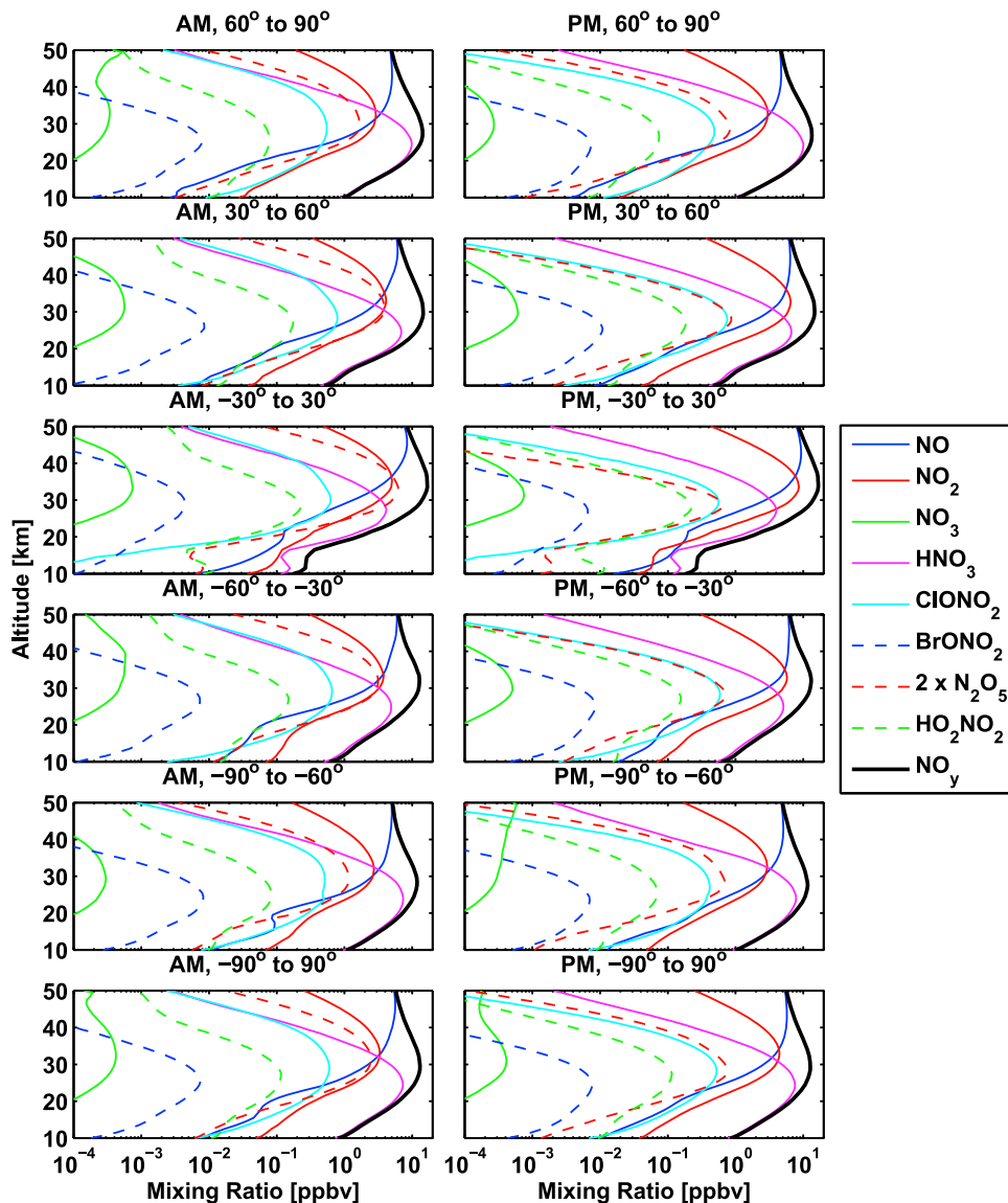
Figure 1. Modeled NO y and individual contributing species average profiles during AM and PM time for six different latitude bands: 60°N–90°N, 30°N–60°N, 30°N–30°S, 30°S–60°S, 60°S–90°S, and 90°S–90°N. Data synthesized by a photochemical box model (see text). The results shown here use simulations made at the time and location of each ACE occultation between 2004 and 2009 with one simulation for each occultation.
