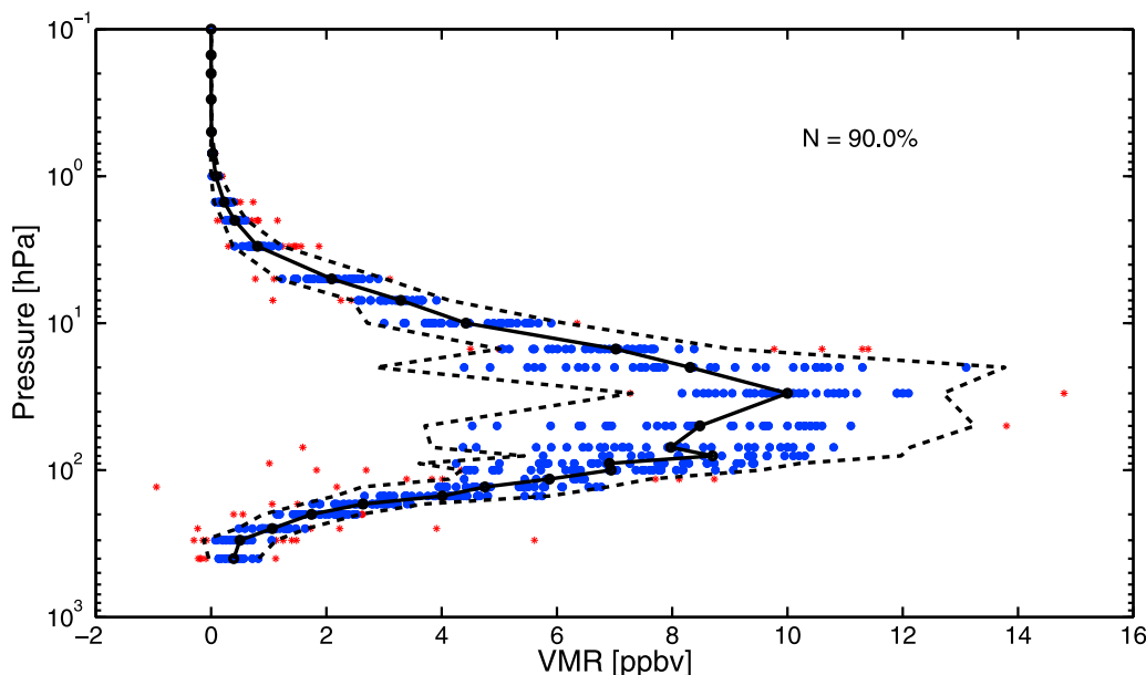
Figure 4. Example of February HNO 3 data (70°N–75°N bin, blue dots) and how outliers are removed using MAD filtering. Red stars are deemed nonrepresentative (~10%) and are thus rejected. The solid black line is the median of all observations, while the dashed line is the three-MAD envelope. N represents the percentage of retained measurements after three-MAD filtering. Here, 10% are removed.
