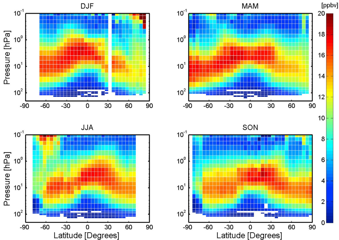
Figure 11. Three month NO y * climatological fields: December–January–February (DJF), March–April–May (MAM), June–July–August (JJA), September–October–November (SON). Values are given in ppbv.
