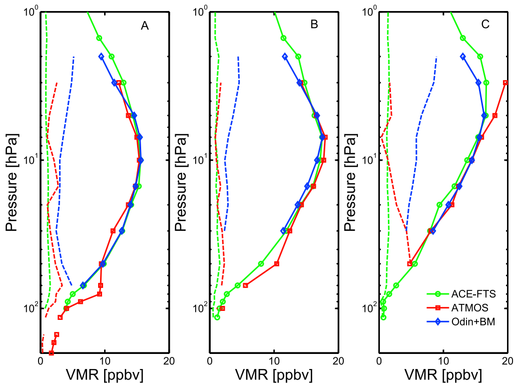
Figure 14. Comparison of mean ACE-FTS, ATMOS, and Odin + box model NO y climatology profiles for three latitude bins: (a) 60°S–70°S (November), (b) 40°S–50°S (March), and (c) 15°N–35°N (April). Dashed lines indicate the 1-sigma spread of the individual measurements from each instrument at each altitude.
