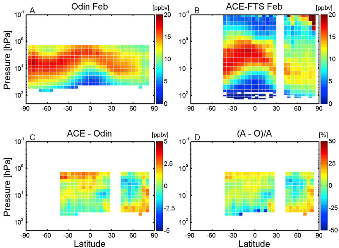
Figure 12. Comparison of the (a) Odin + box model NO y and (b) ACE-FTS NO y * climatologies for the month of February. Also shown are the (c) absolute deviations given in ppbv and (d) relative differences ((ACE-Odin)/ACE), given in percent.
