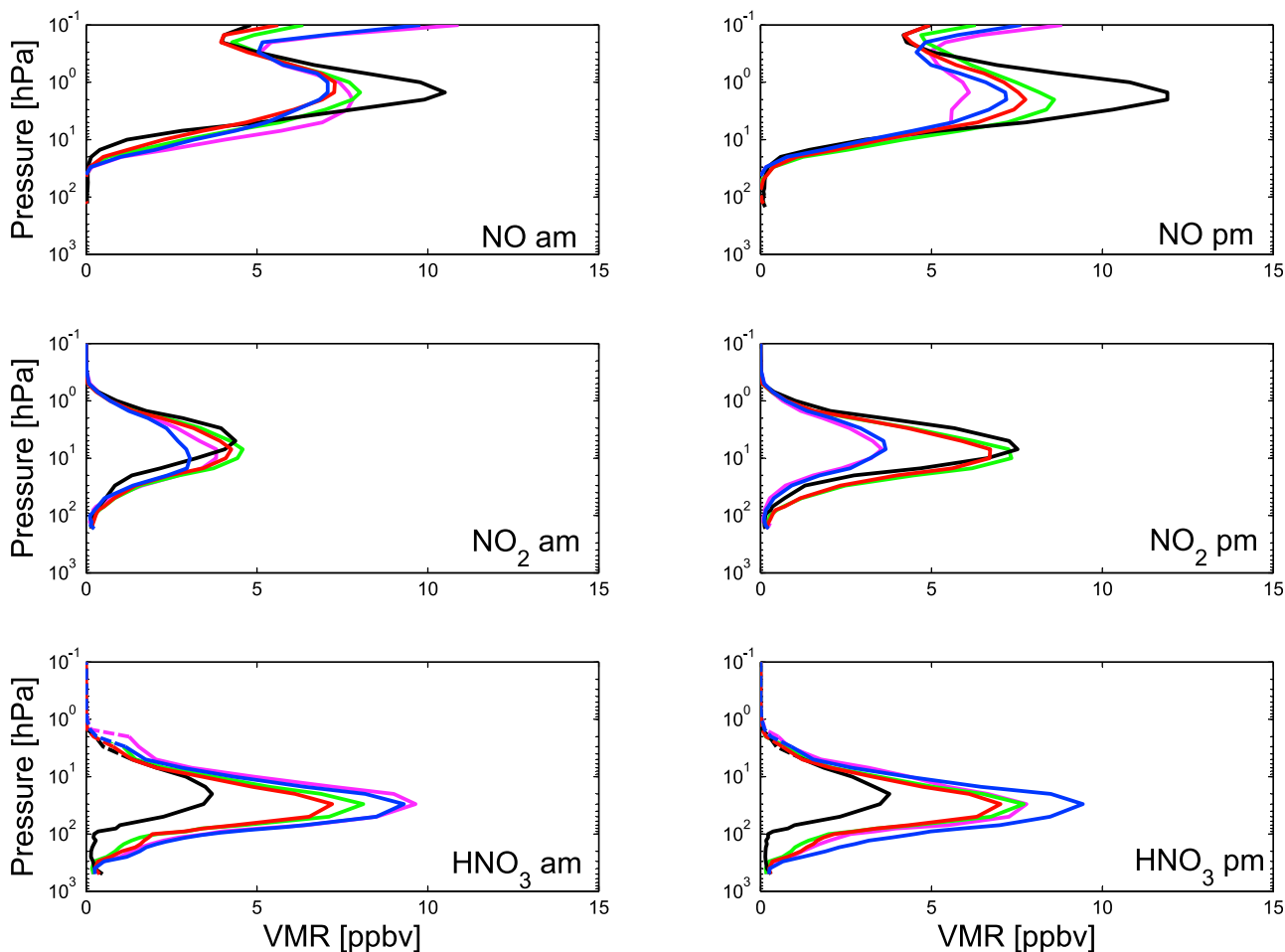
Figure 7a. Median VMR profiles of NO, NO 2 , and HNO 3 in five latitude bands using ACE-FTS data from February 2004 to February 2009. (left) AM observations. (right) PM observations. Latitude bands are coded as: blue, 60°N–90°N; red, 30°N–60°N; black, 30°N–30°S; green, 30°S–60°S; pink, 60°S–90°S. Solid lines are measurements, and dashed lines are where only scaled initial guess values are considered.
